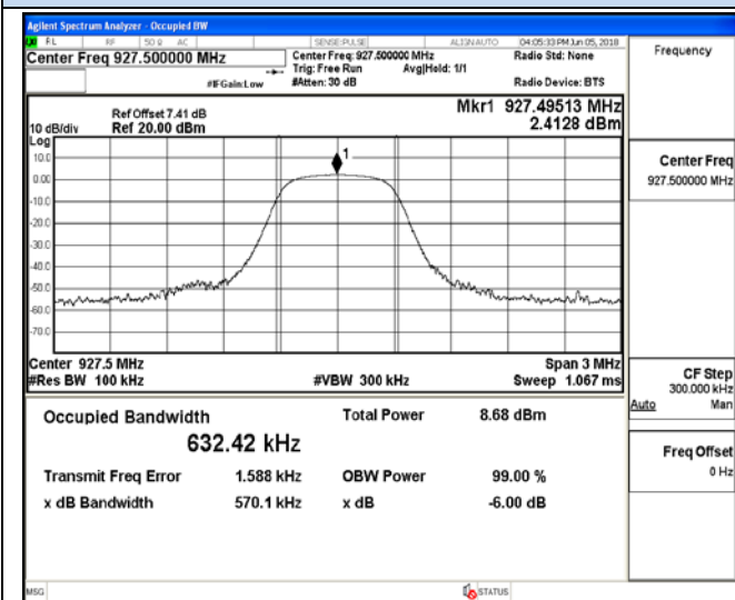
Channel 10 / 927.5 MHz
