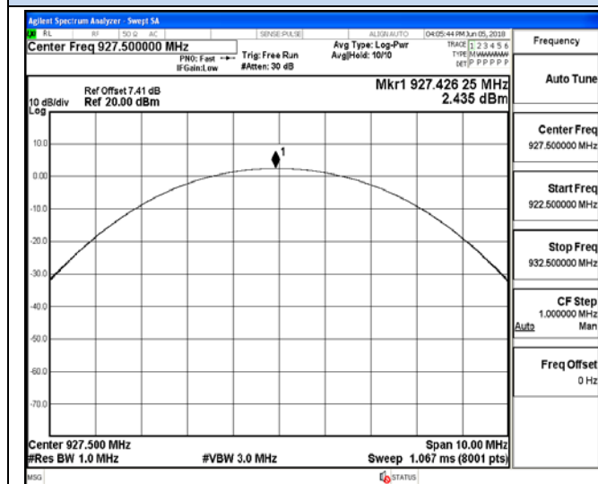
Channel 10 / 927.5 MHz
