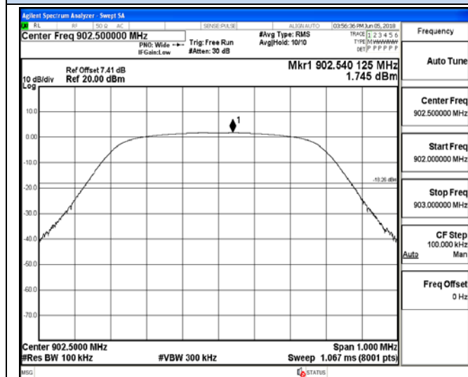
Channel 0 / 902.5 MHz
