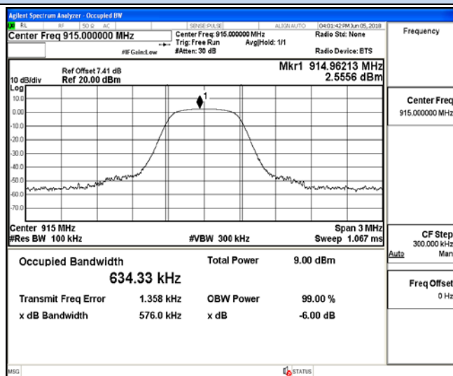
Channel 05 / 915 MHz
