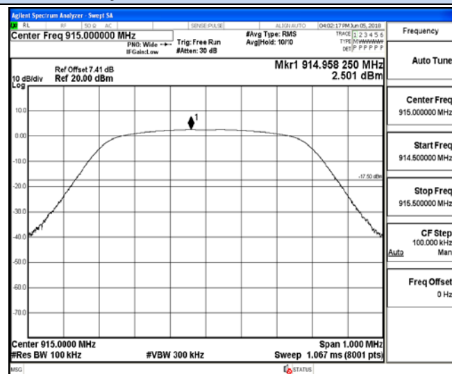
Channel 05 / 915 MHz
