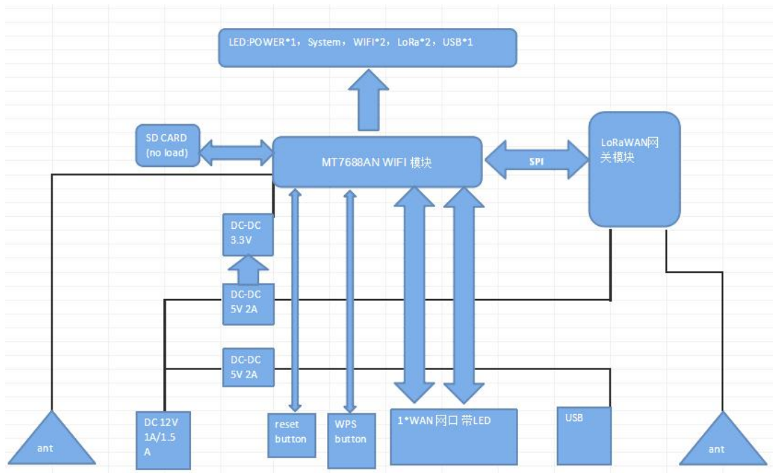
Figure 2- 1 GW200 functional block
