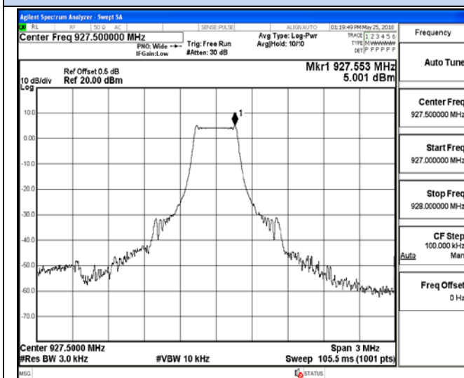
Channel 10 / 927.5 MHz
