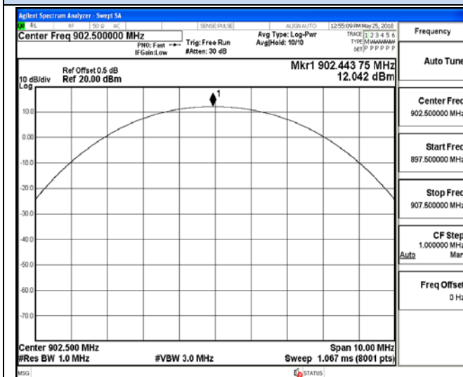
Channel 0 / 902.5 MHz
