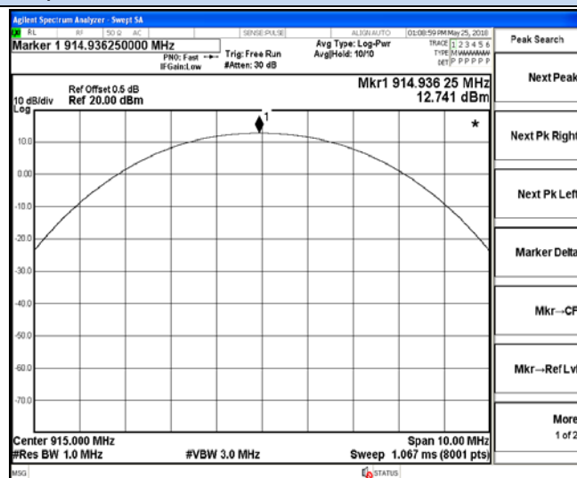
Channel 05 / 915 MHz
