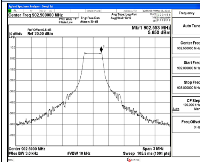
Channel 0 / 902.5 MHz
