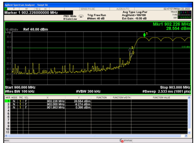
Hopping mode
