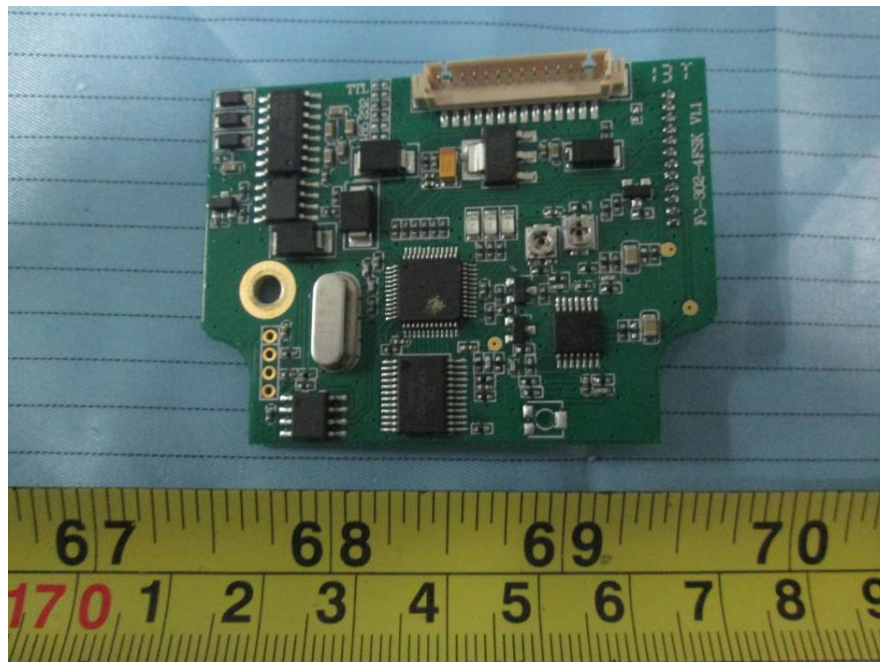
EUT –4FSK Board Top View
