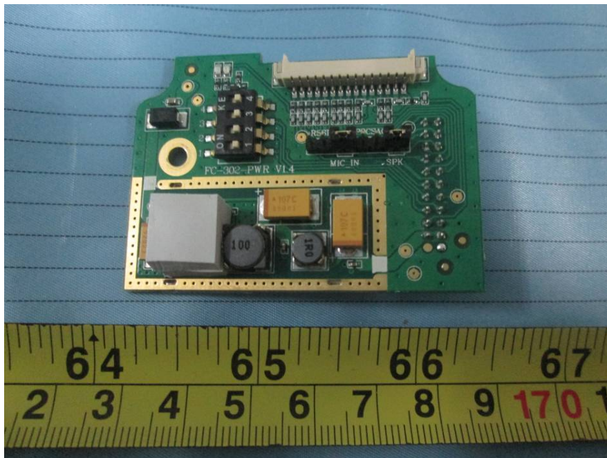
EUT –PCB 302 Top Shielding off View
