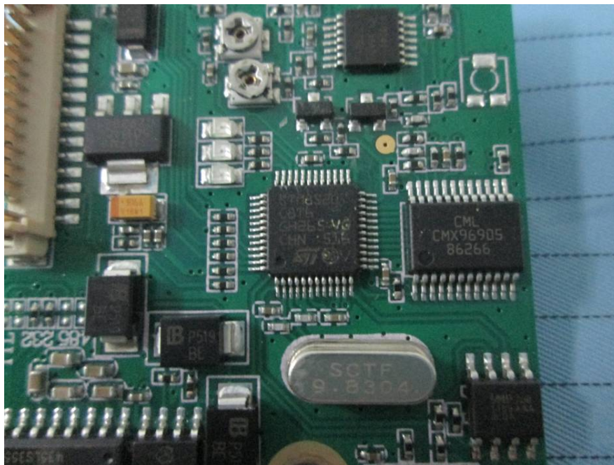
EUT -4FSK Main IC View
