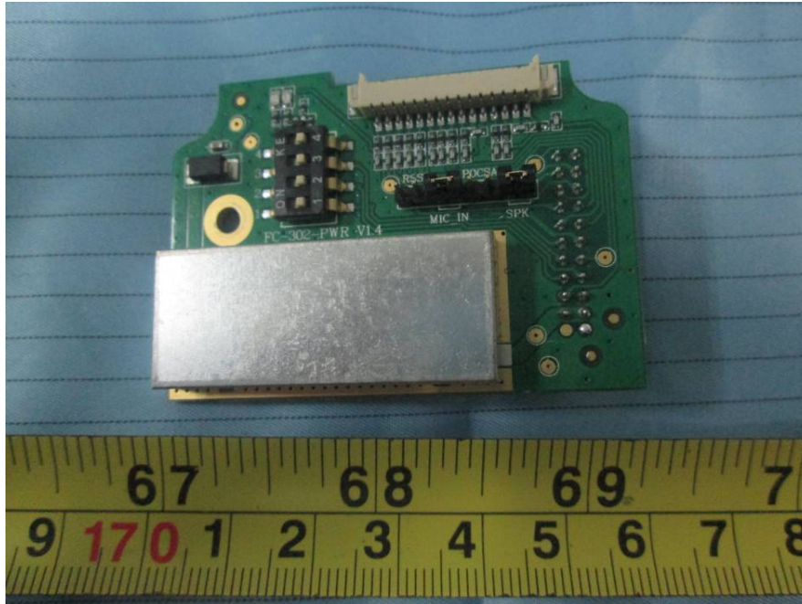
EUT –PCB 302 Top View
