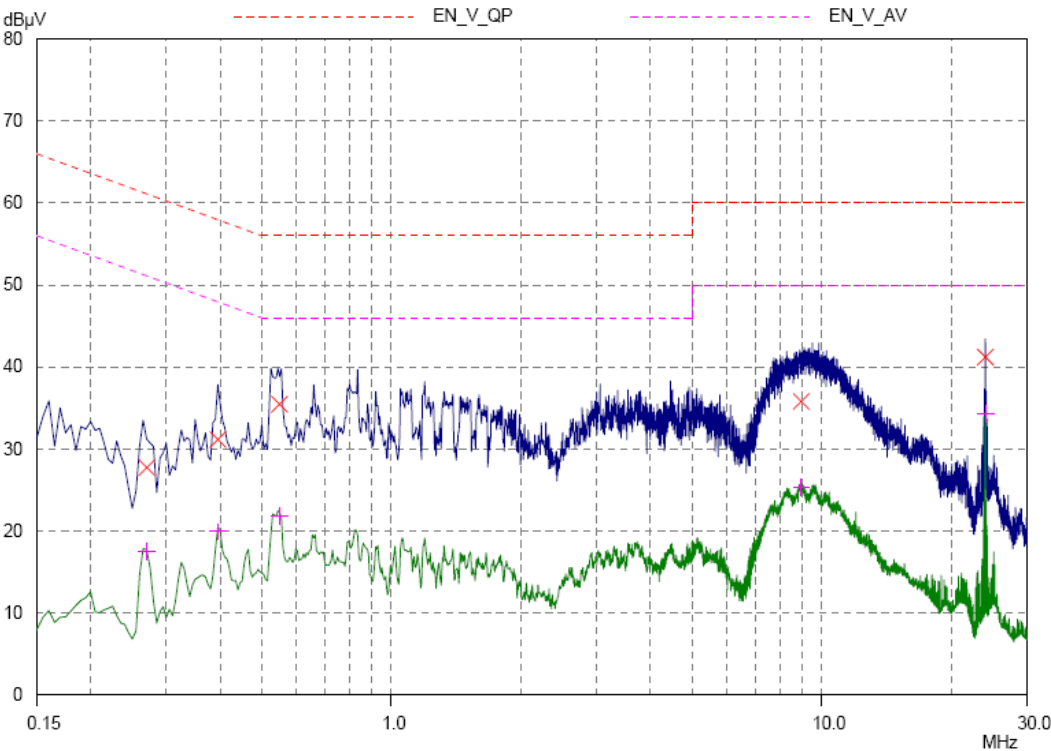
Figure 11. Plot of the Conducted Emissions
