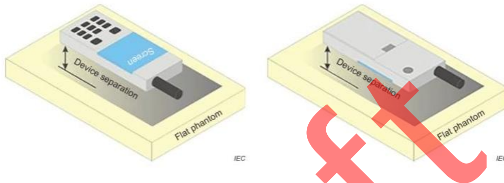
Figure 6 – Test positions for body-worn devices
