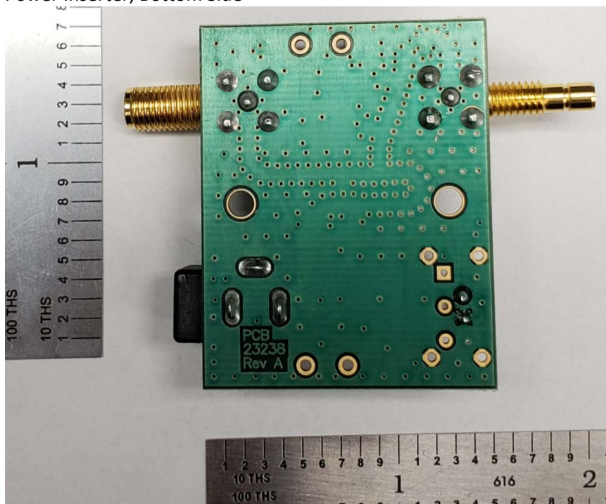
Power Inserter, Bottom Side
