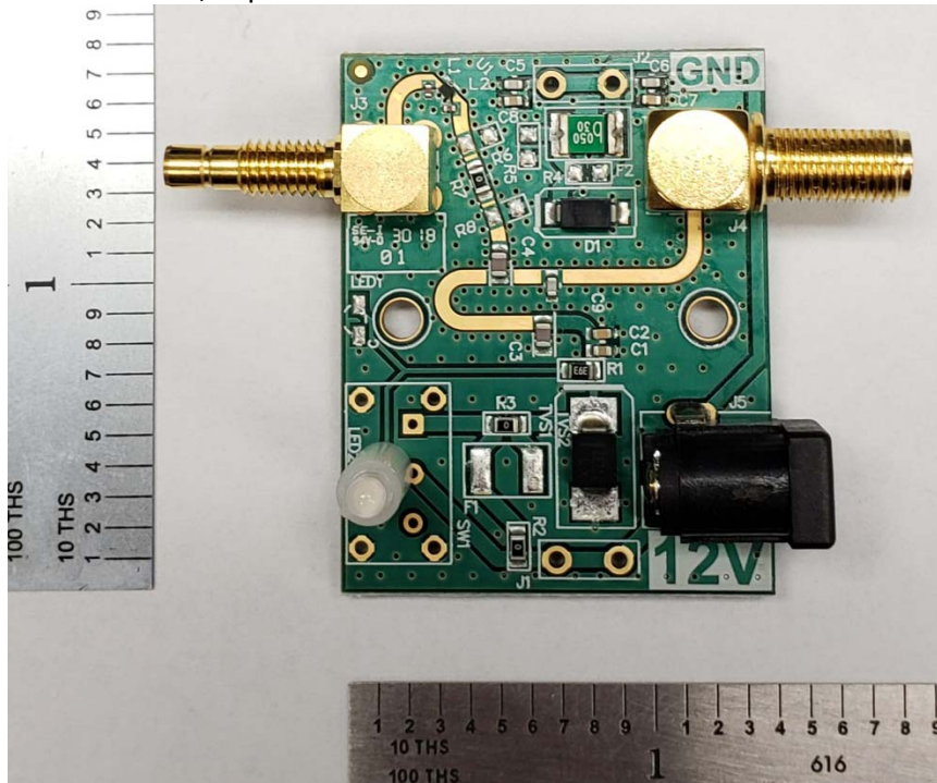
Power Inserter, Top Side
