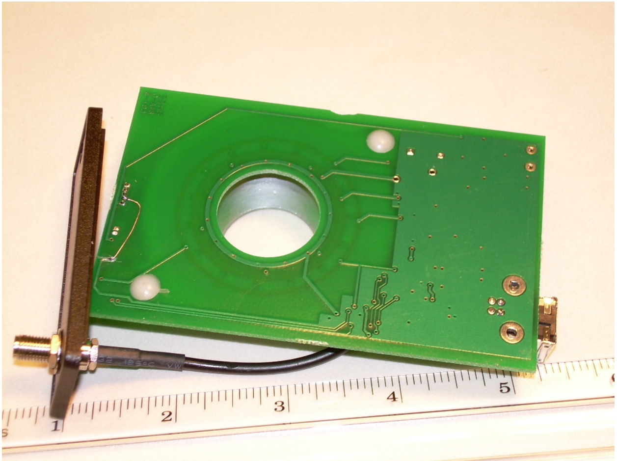
View of the Trace Side of the MPRF-H PCB
