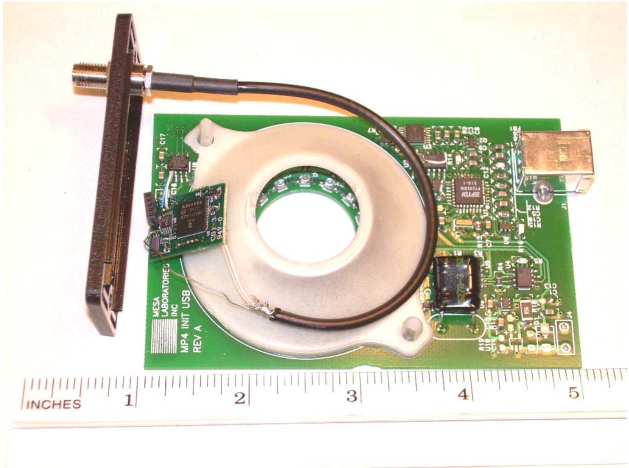
View of the Component Side of the MPRF-H PCB
