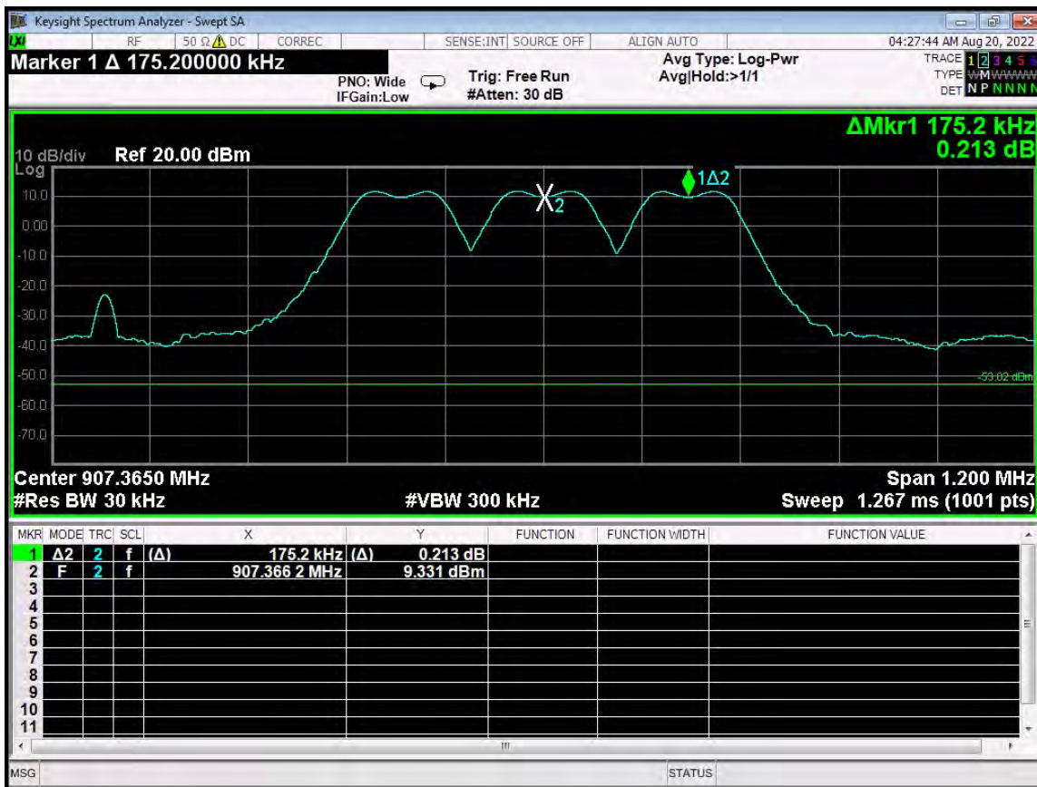
Channel Frequency Separation - Hop Set 2 - G4 Compatibility Mode
