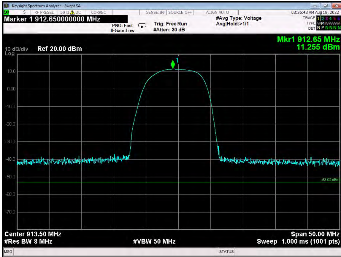
Peak Power Output - 913.50 MHz - G4 Compatibility Mode
