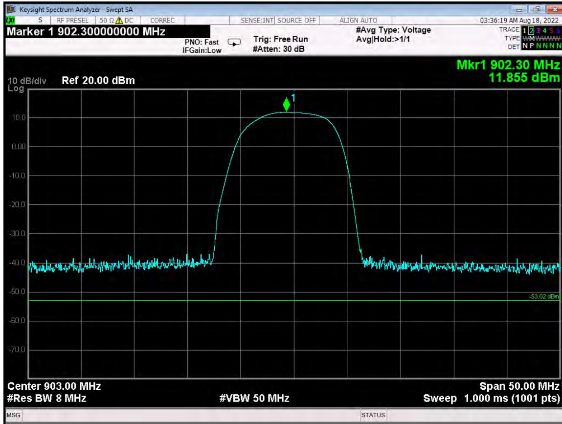
Peak Power Output - 903.00 MHz - G4 Compatibility Mode
