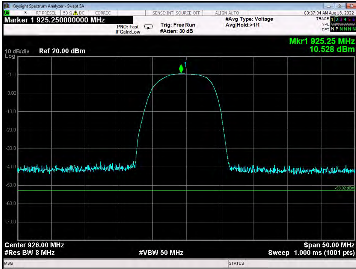
Peak Power Output - 926.00 MHz - G4 Compatibility Mode
