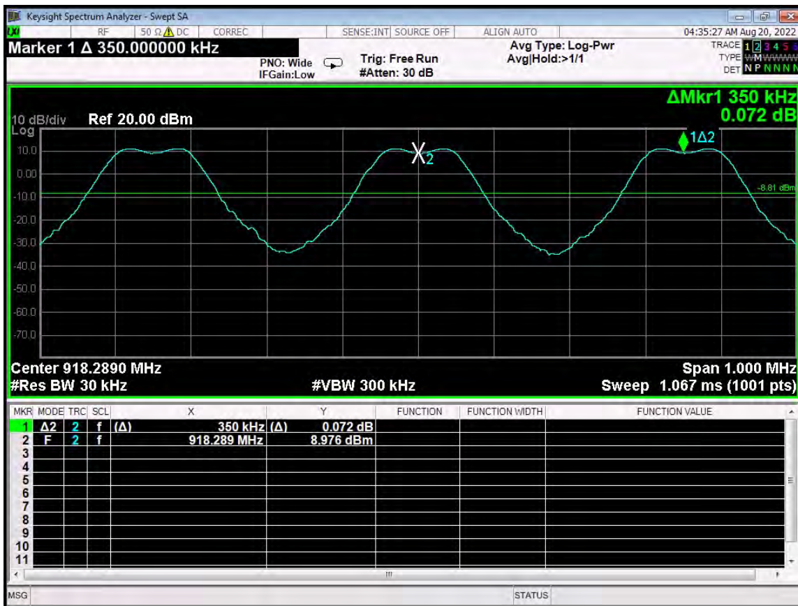
Channel Frequency Separation - Hop Set 1 - G4 Compatibility Mode
