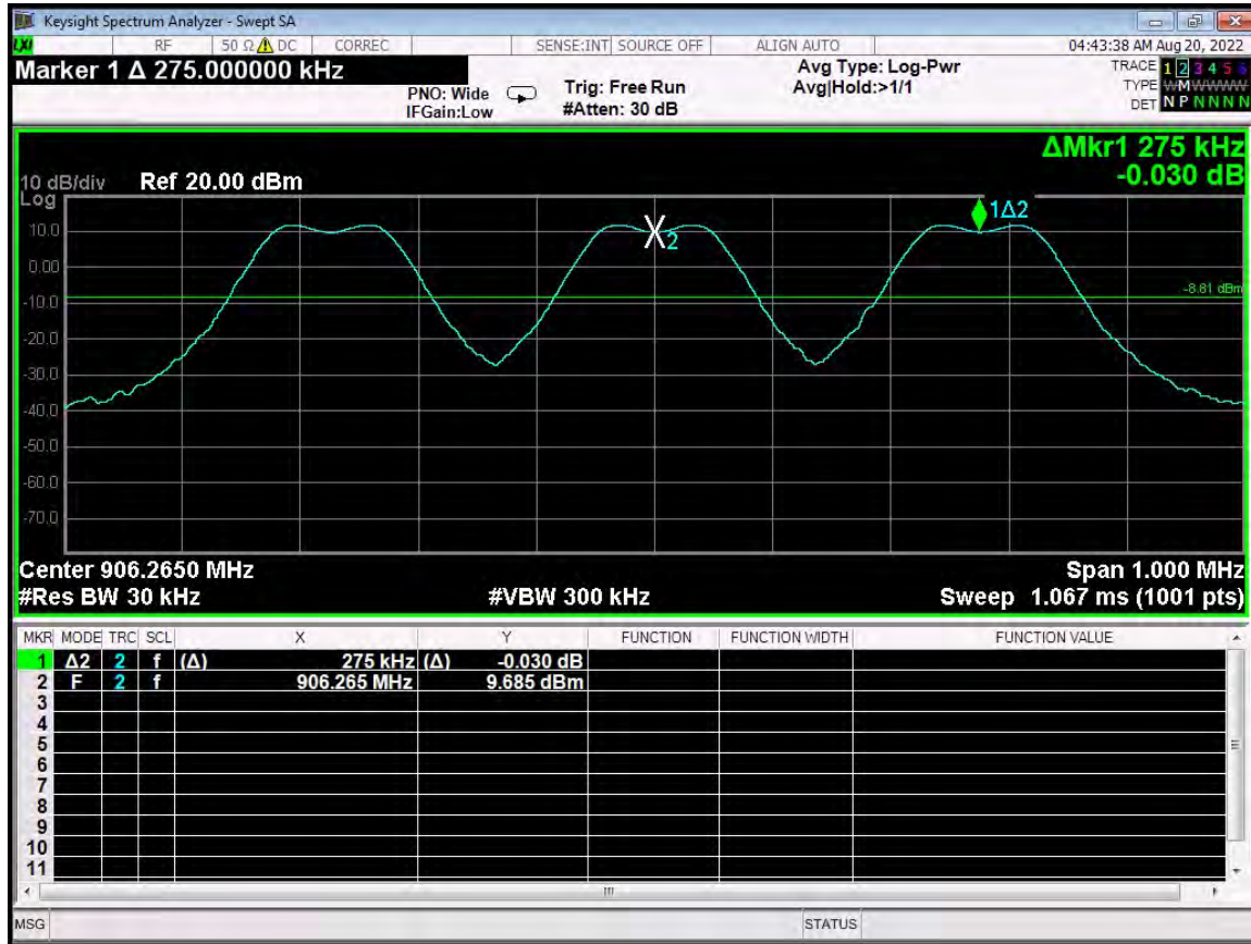
Channel Frequency Separation - Hop Set 0 - G4 Compatibility Mode
