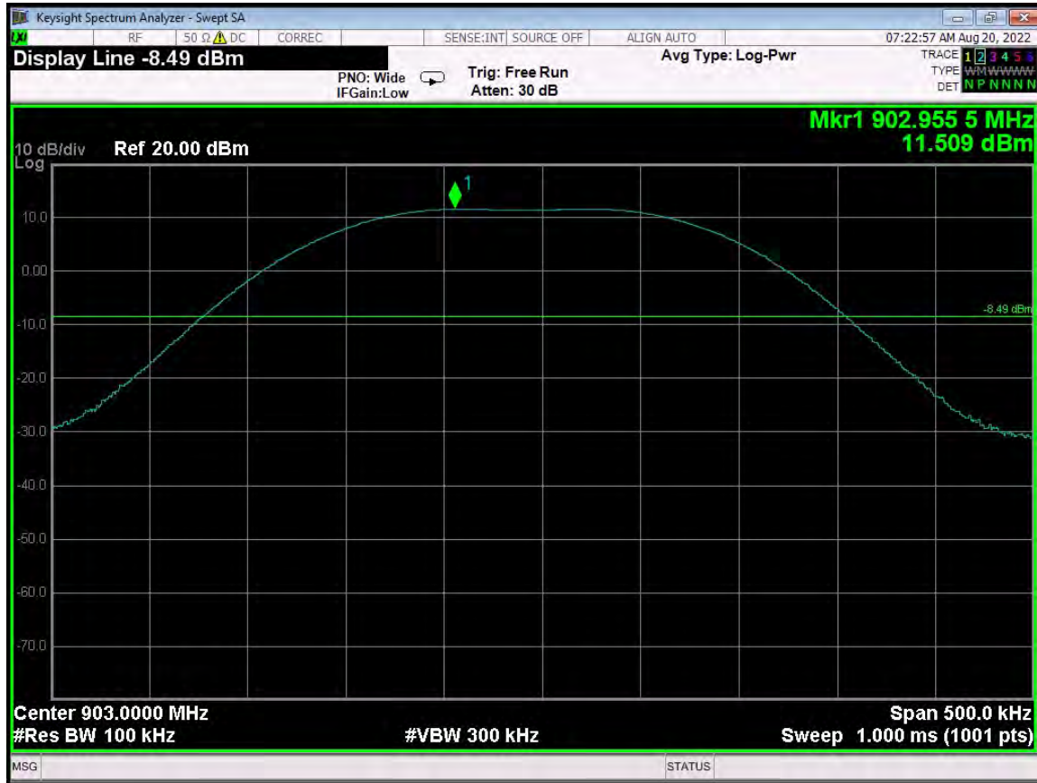
RF Antenna Conducted Low Channel - G4 Compatibility Mode - Reference Level
