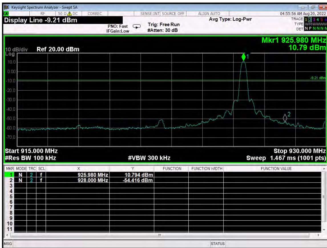
High Channel - G4 Compatibility Mode - Single Channel
