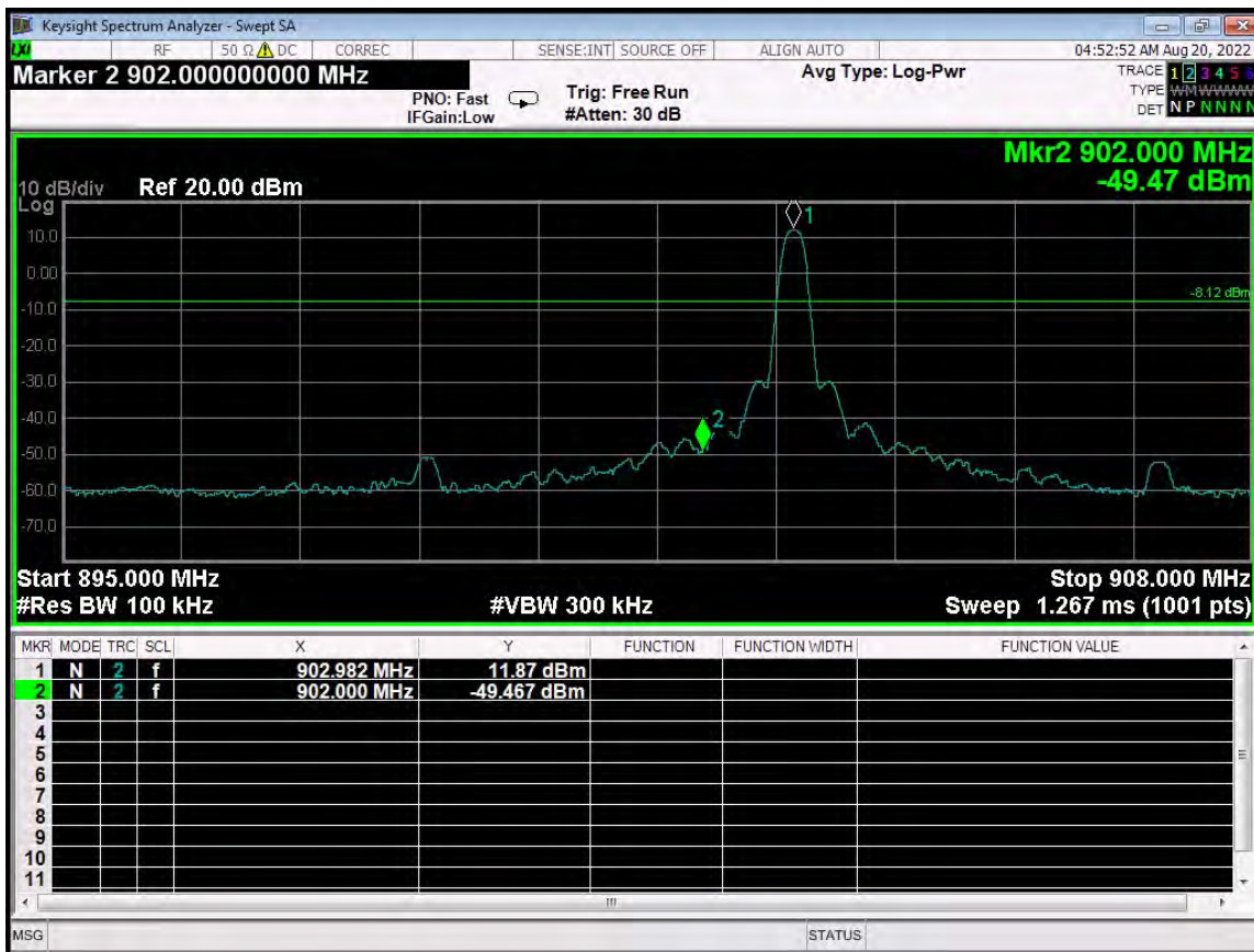
Band Edge – Low Channel - G4 Compatibility Mode - Single Channel
