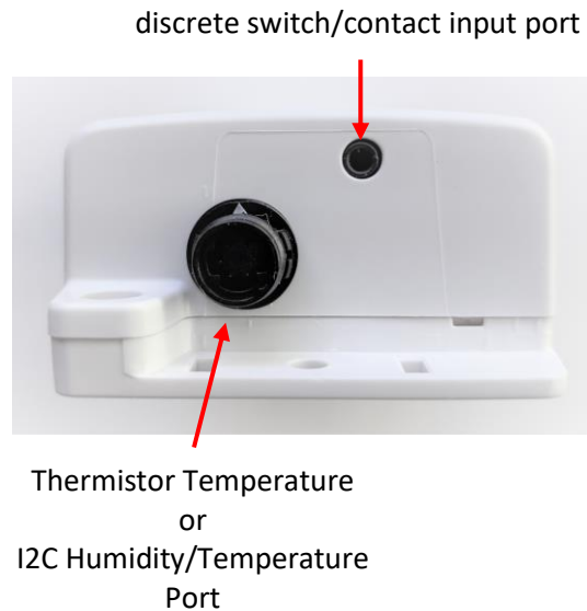
6-2 VP Essentials Sensor Top Side View Showing Ports
