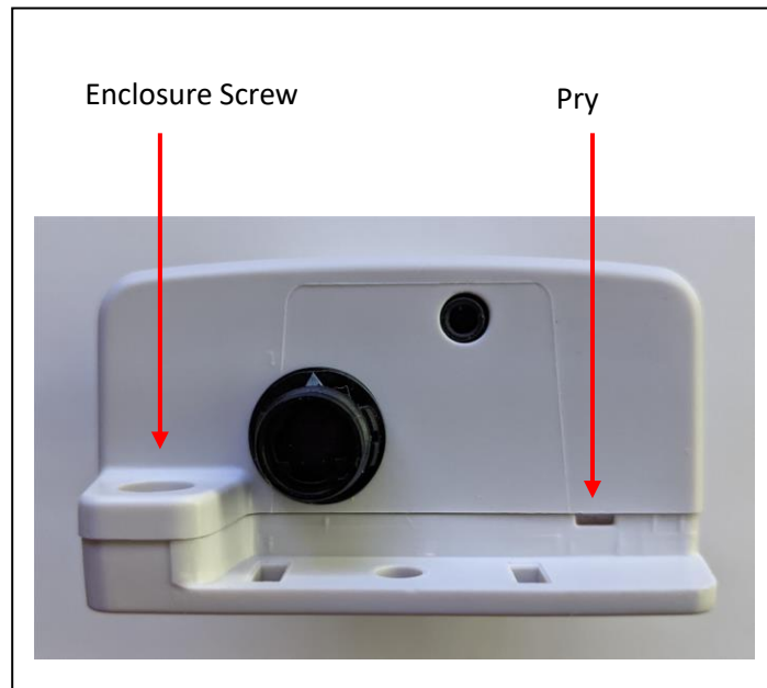
7-1 VP Essentials Sensor – Opening Enclosure
