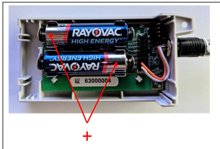
7-1 VP Essentials Sensor – Batteries
