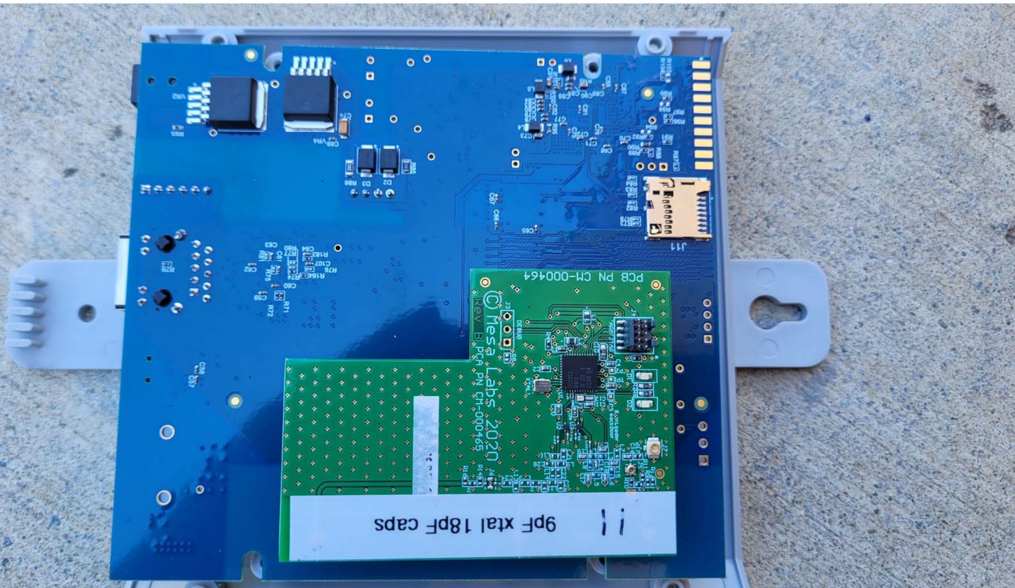
Bottom View of the PCB with RF Board
