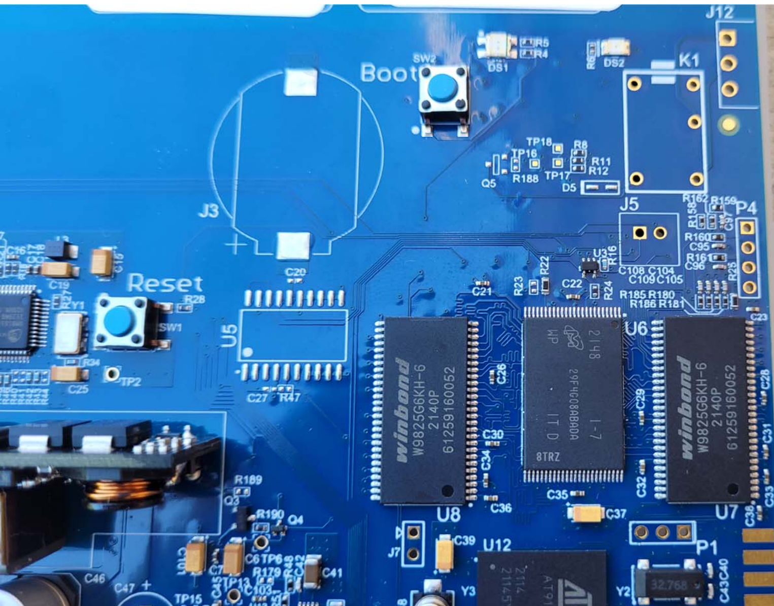
Top View of the PCB - Closeup #3
