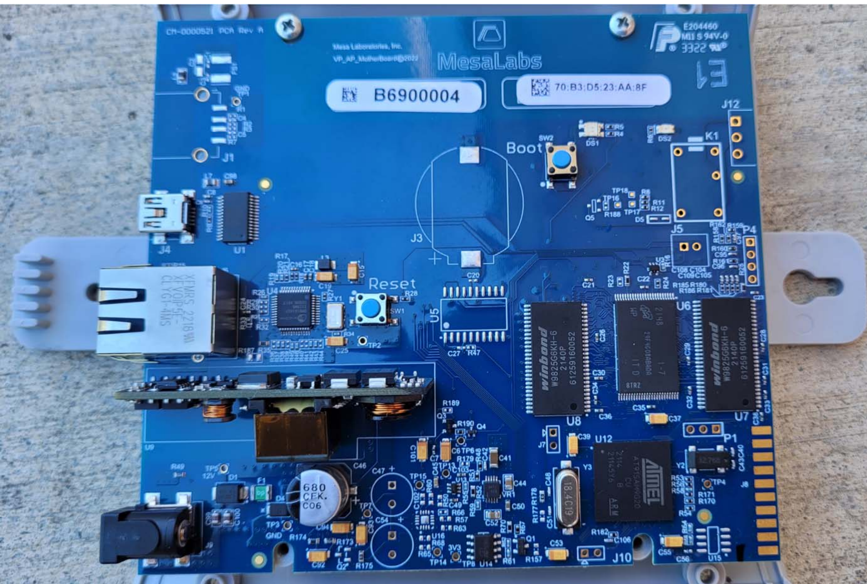
Top View of the PCB for the EUT
