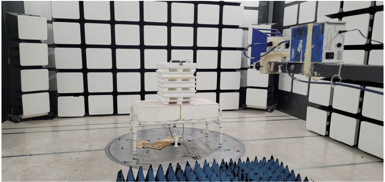
FRONT VIEW
