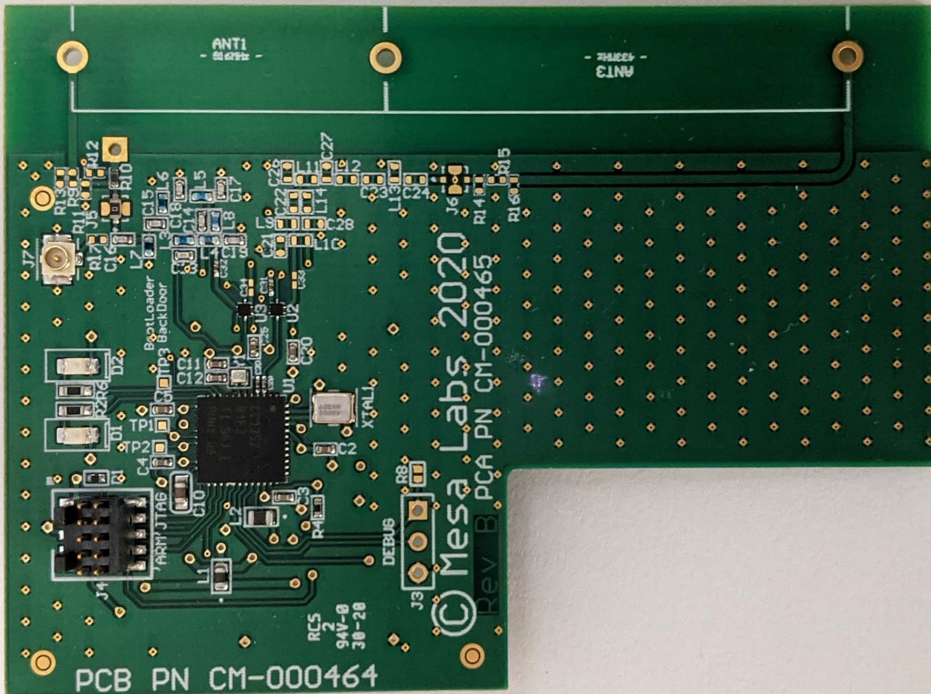
Top View of the RF Module
