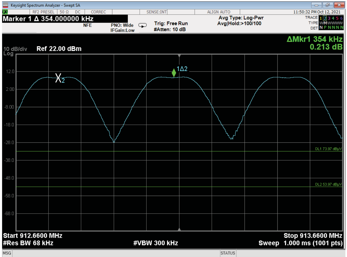
Channel Frequency Separation – Hop Set 1
