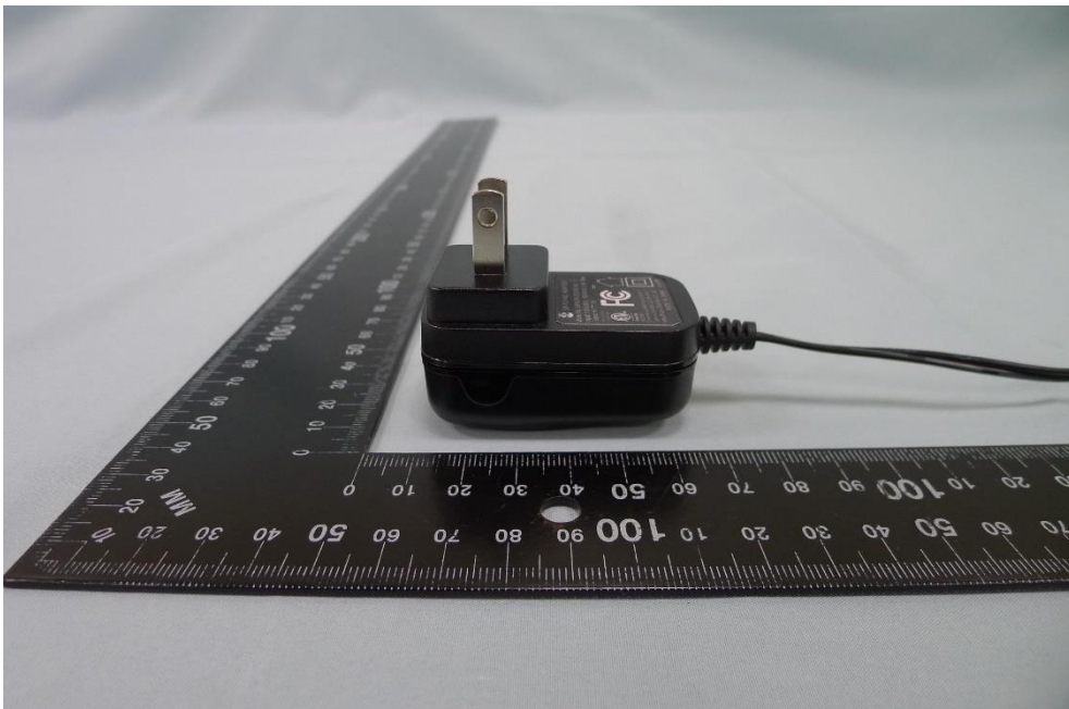
(12) Adapter Photo
