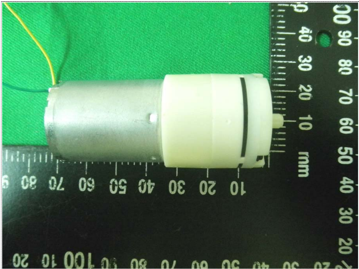
Rear View of pump
