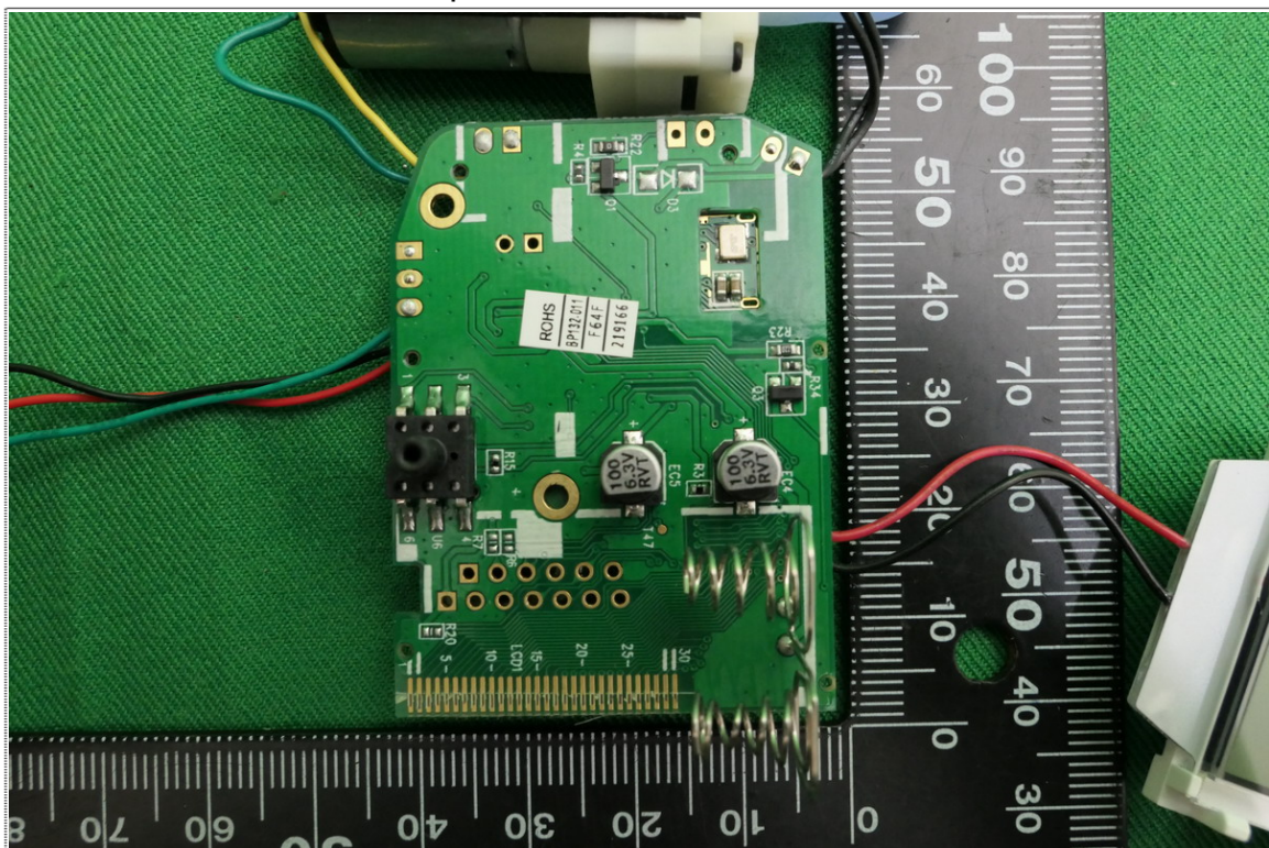
Solder View of Main Board-1
