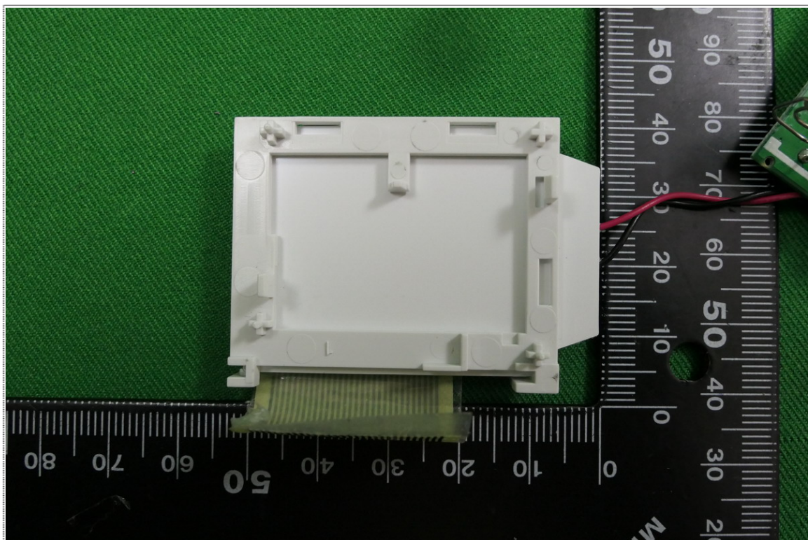
Rear View of Panel
