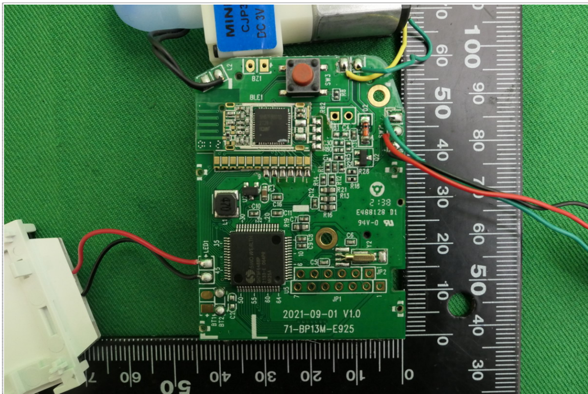
Component View of Main Board-1
