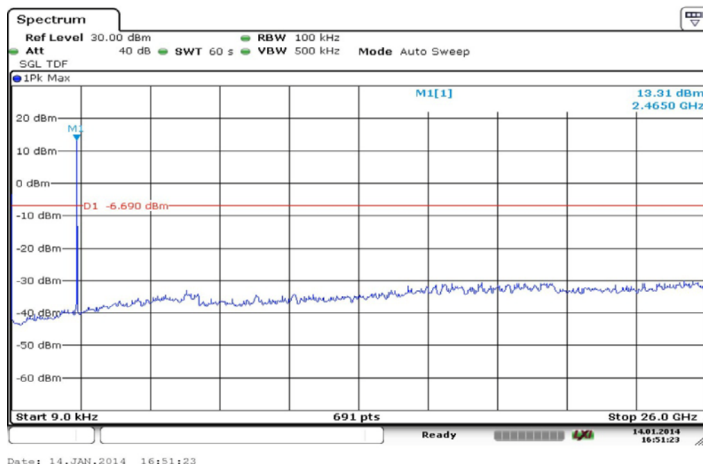
Plot 2: TX mode, middle channel, up to 26 GHz
