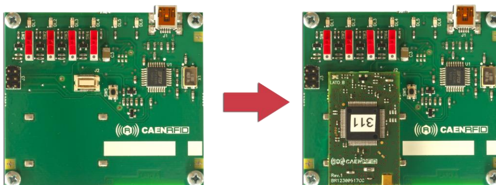
Fig. 1.5: Connection of the R1230CBEBV to the Quark R1230CB module
