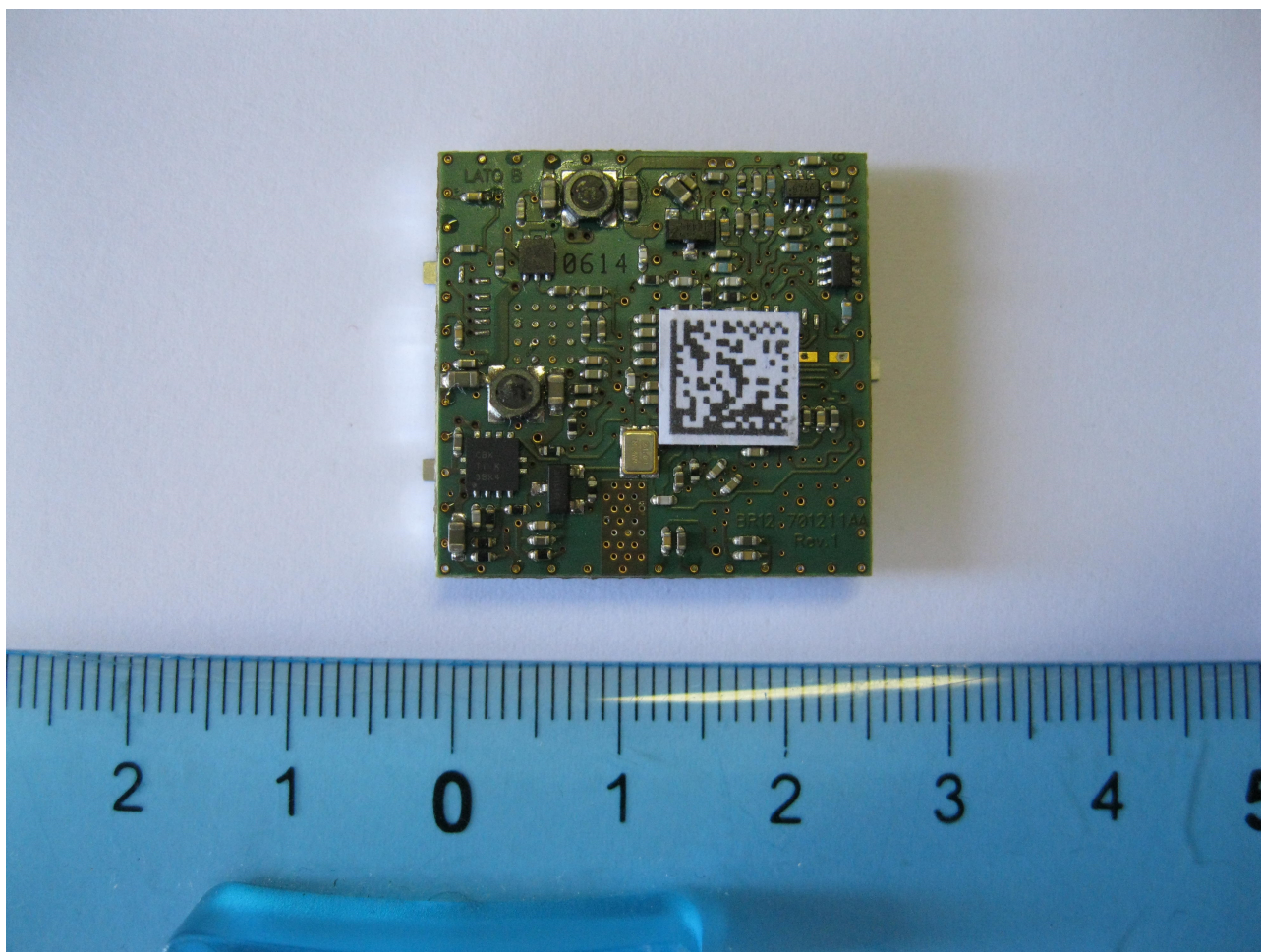
Figure 2 - R1270C Module Bottom View
