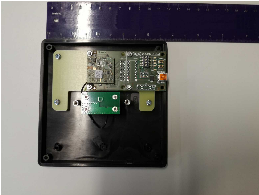
Figure 5 - R1270C module connected with 7R1251IUNFAA antenna
