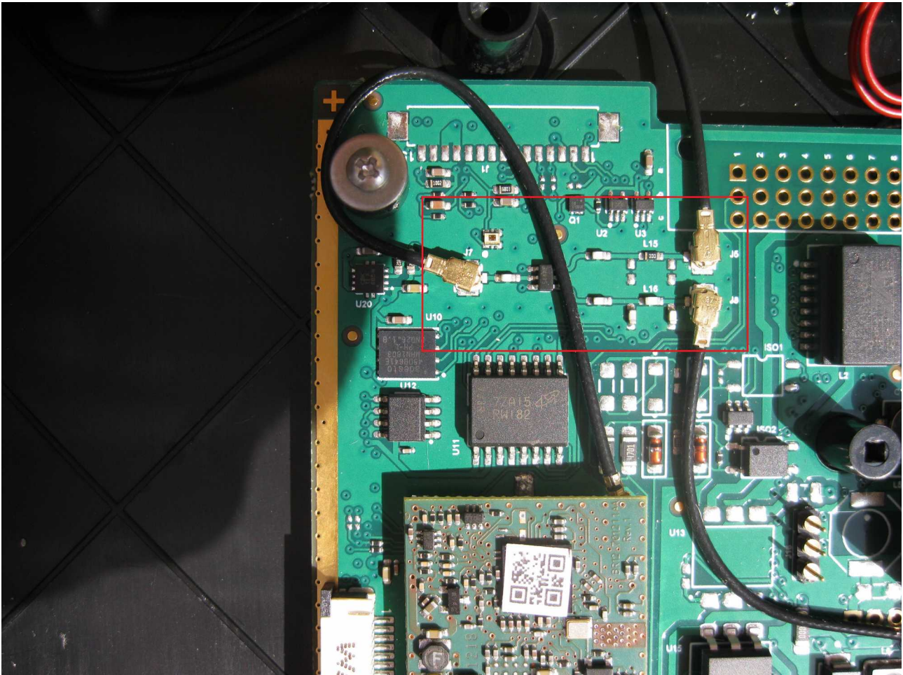
Figure 4 - Zoom on RF switch section
