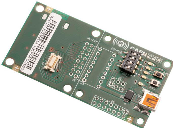
Fig. 1.2: Quark Up R1270CEVB - Quark-Up Reader Evaluation Board
