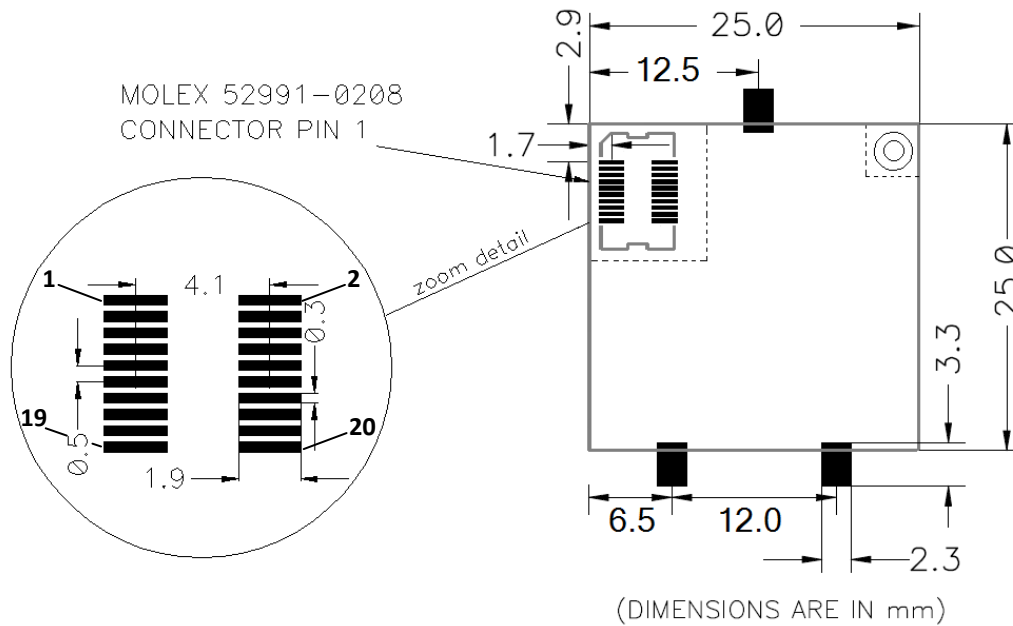
Fig. 2.9: PCB pad layout
