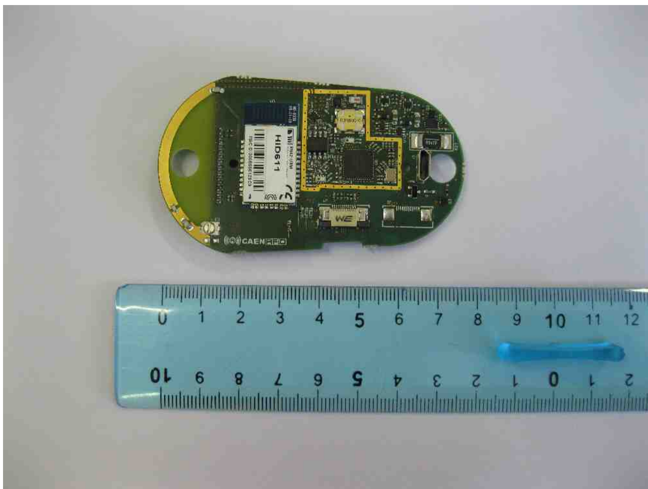
Fig. 6: R1170IUHIDP - PCB Bottom Side
