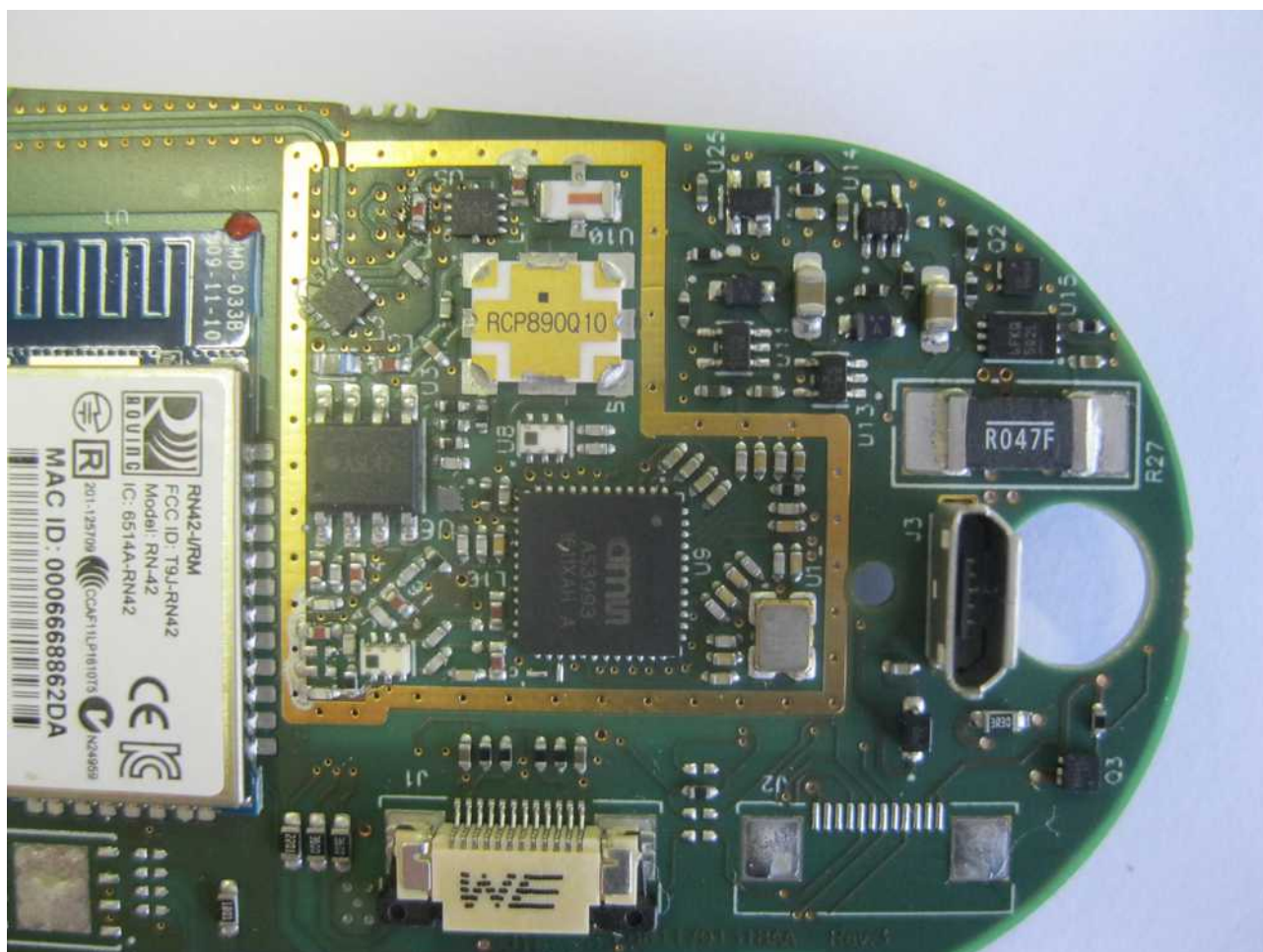
Fig. 6: R1170IUAPLP / R1170IUHIDP - RFID section with shield removed
