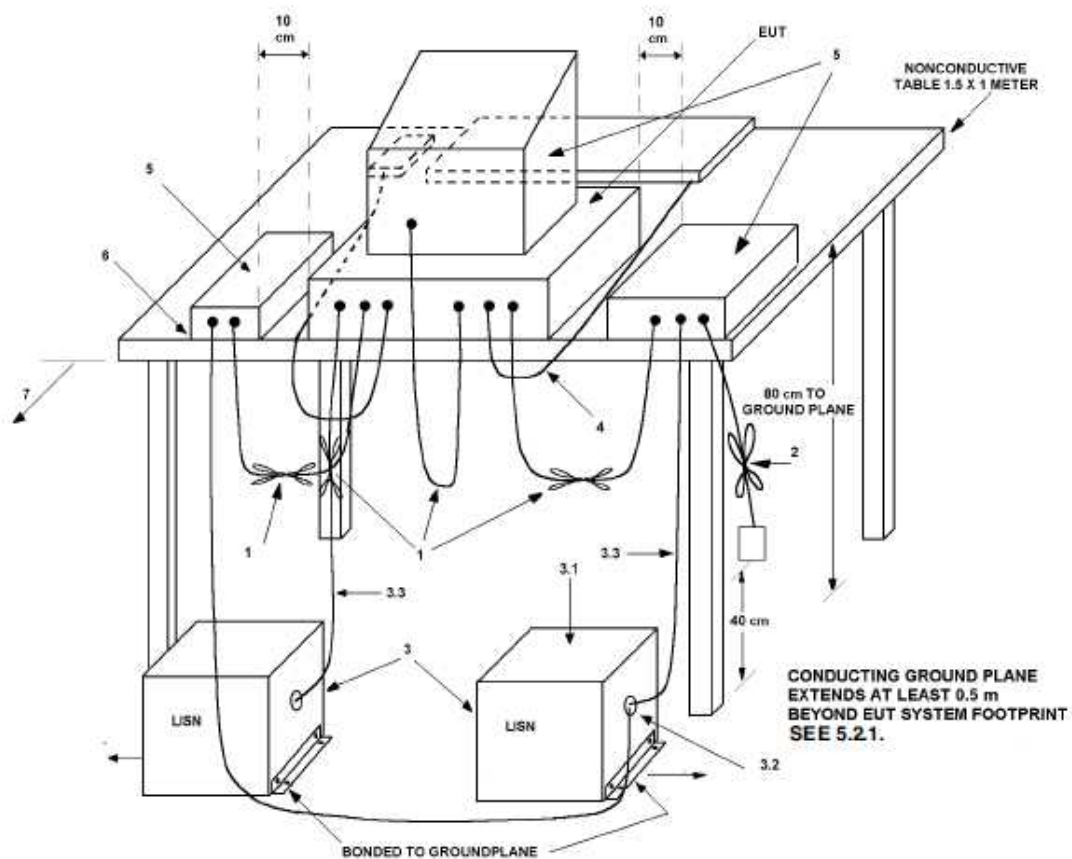
Conducted and Radiated EUT Test Set-up example (ANSI C63.4 2009)
