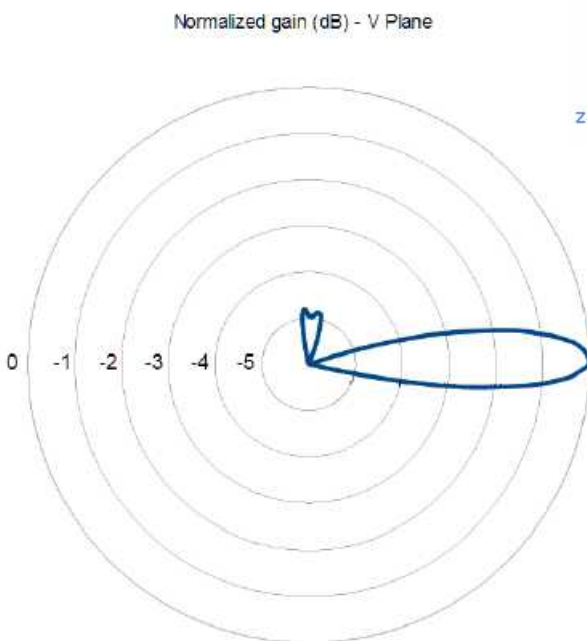
Fig. 8.8: qIDmini R1170IU Radiation pattern V plane
