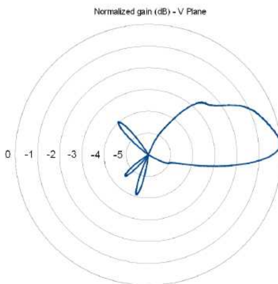
Fig. 8.6: qIDmini R1170IE Radiation pattern V plane
