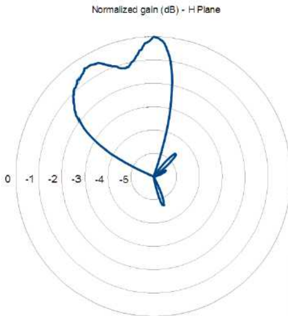
Fig. 8.7: qIDmini R1170IU Radiation pattern H plane
