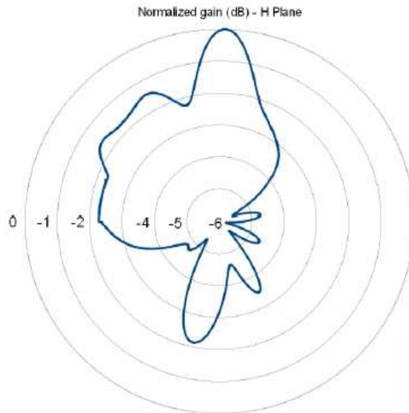
Fig. 8.5: qIDmini R1170IE Radiation pattern H plane
