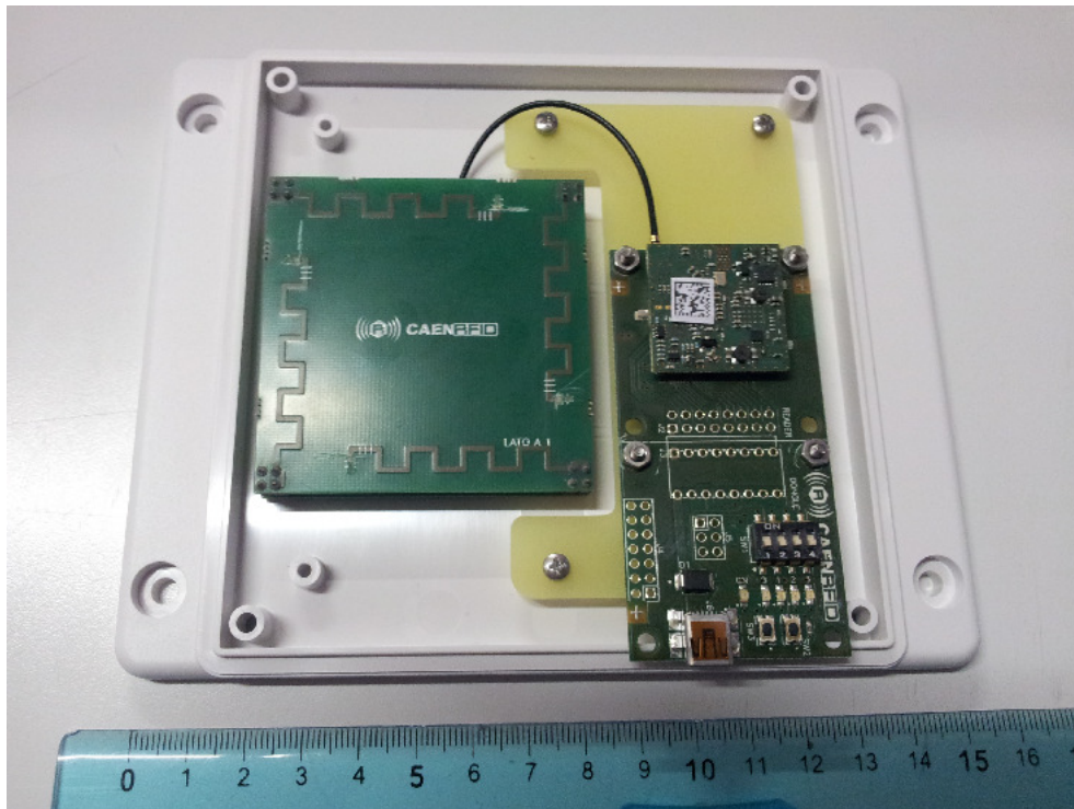
Fig. 25: R1250IUFL – Assembly Internal View
