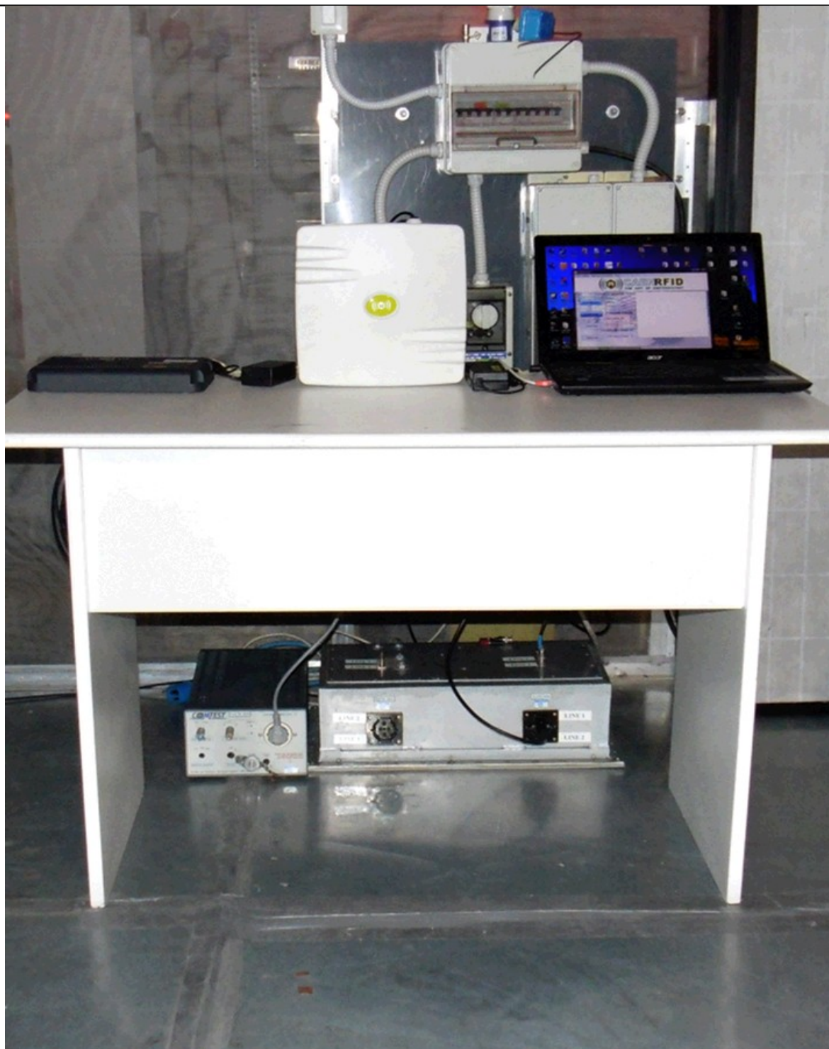
Fig. 6.1 Conducted Emissions Test Set-up
