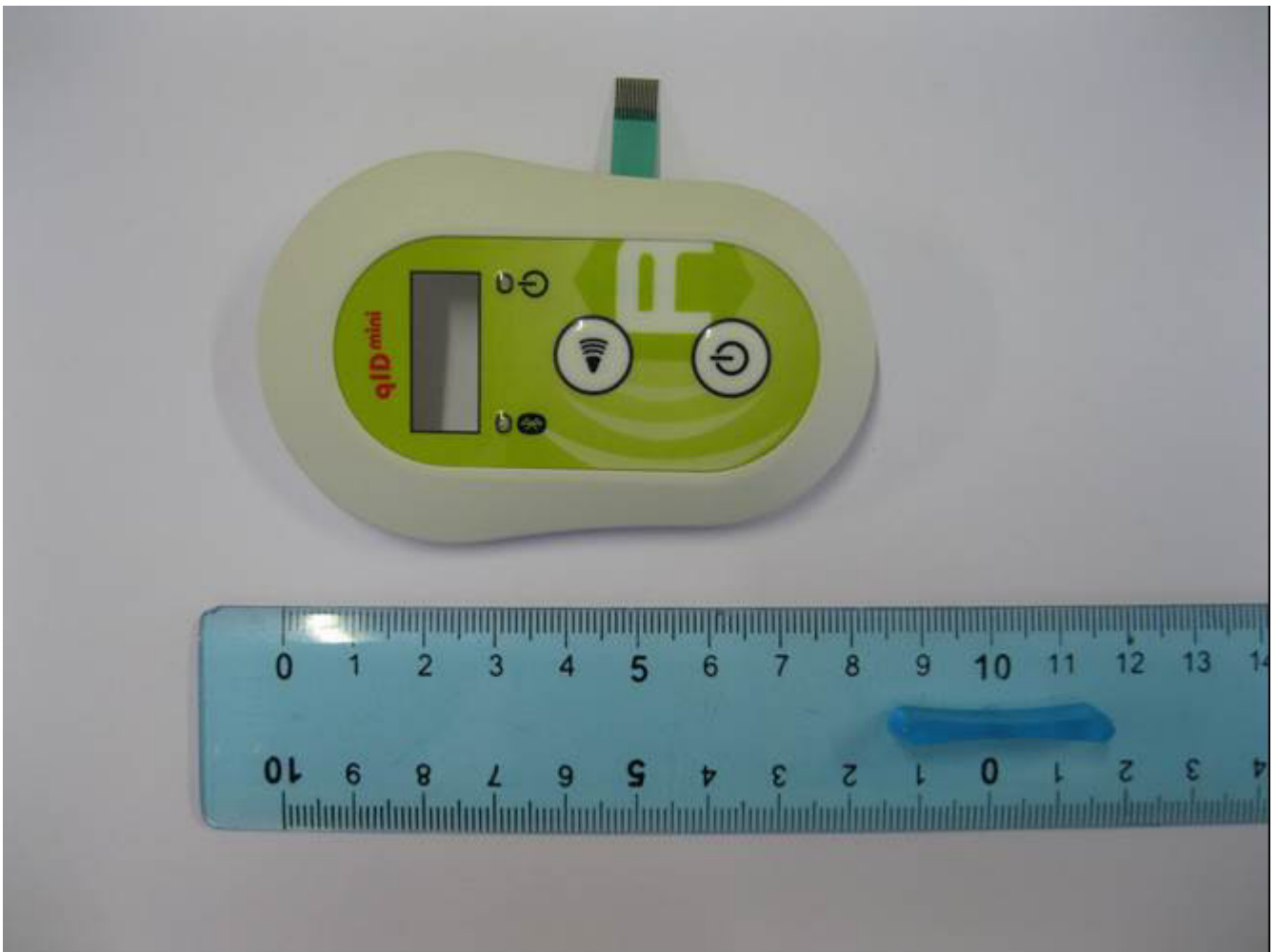
Fig. 5: Enclosure and keypad Top Side (external view)
