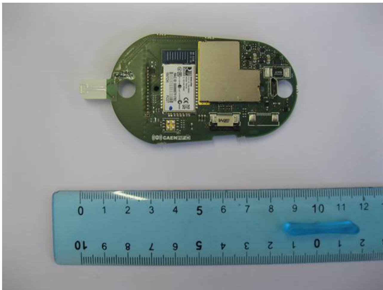
Fig. 4: PCB Bottom Side with shield installed
