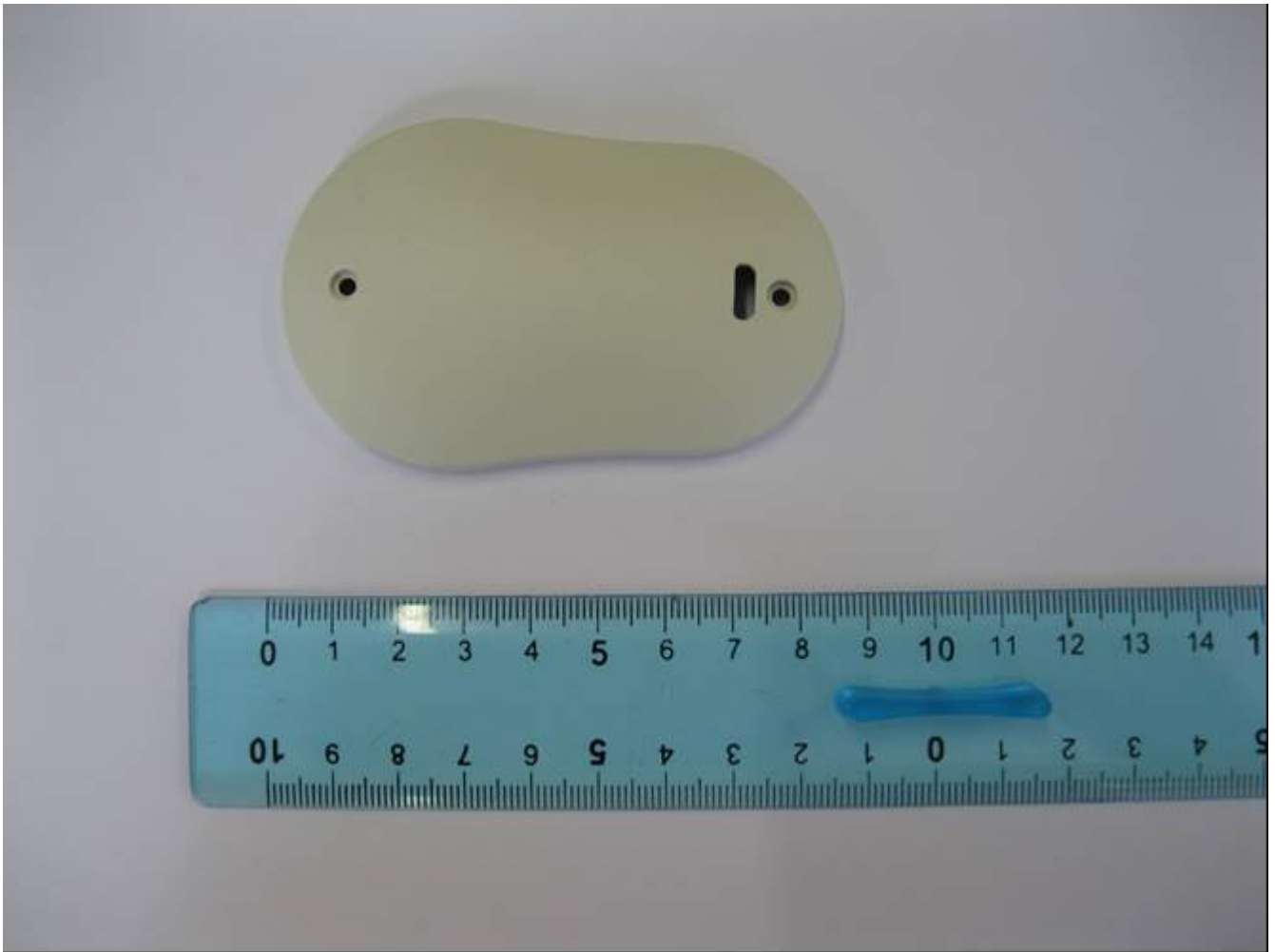
Fig. 8 Enclosure Bottom Side (external view)
