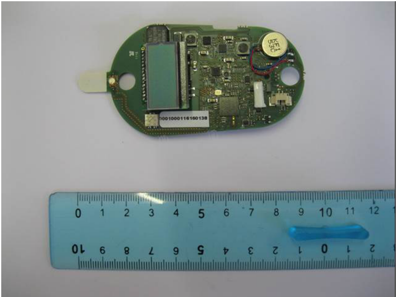
Fig. 3: PCB Top Side with display installed
