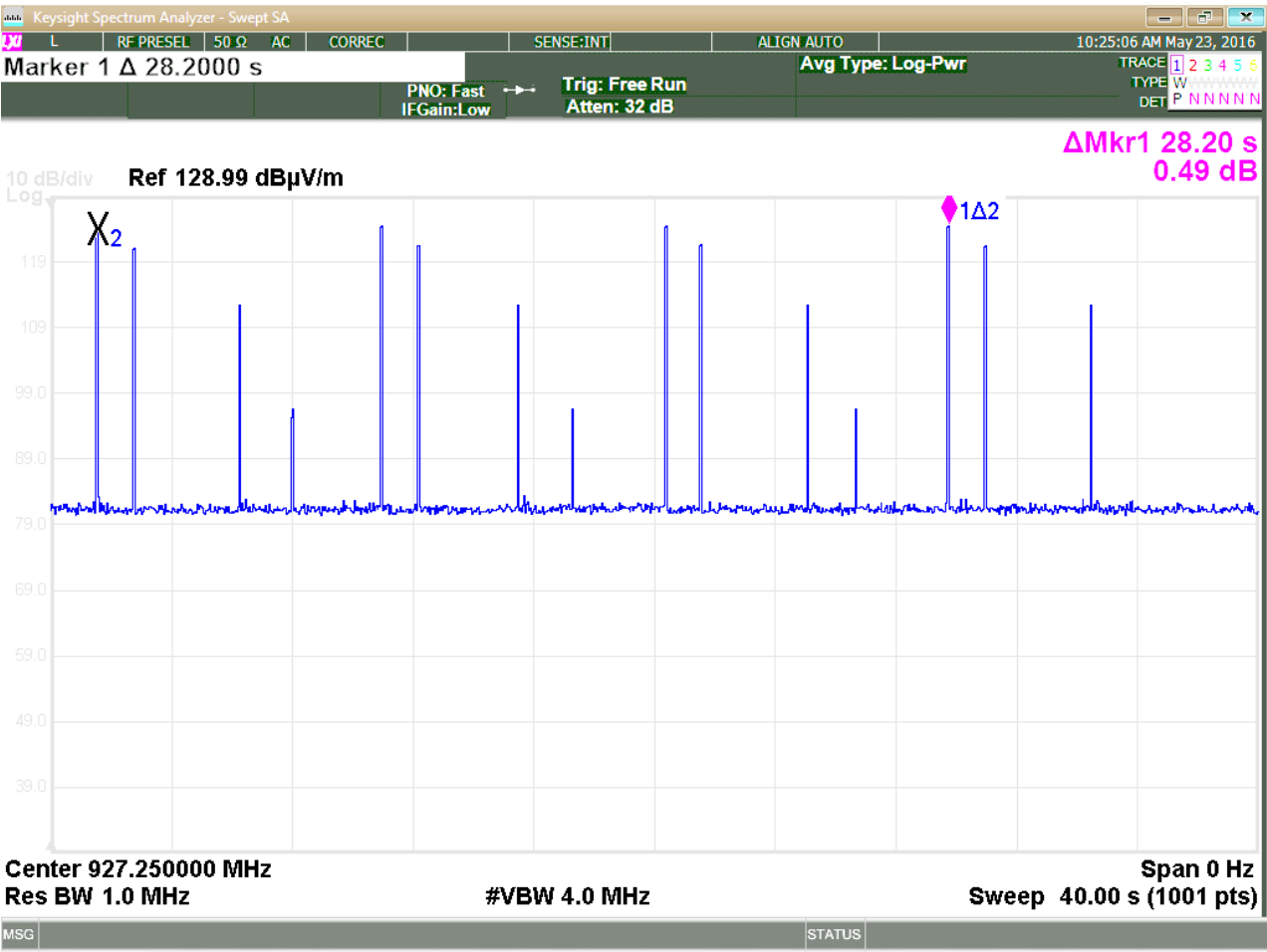
Fig. 6.10 Channel: 49
