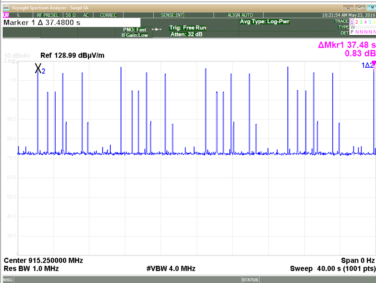
Fig. 6.8 Channel: 25
