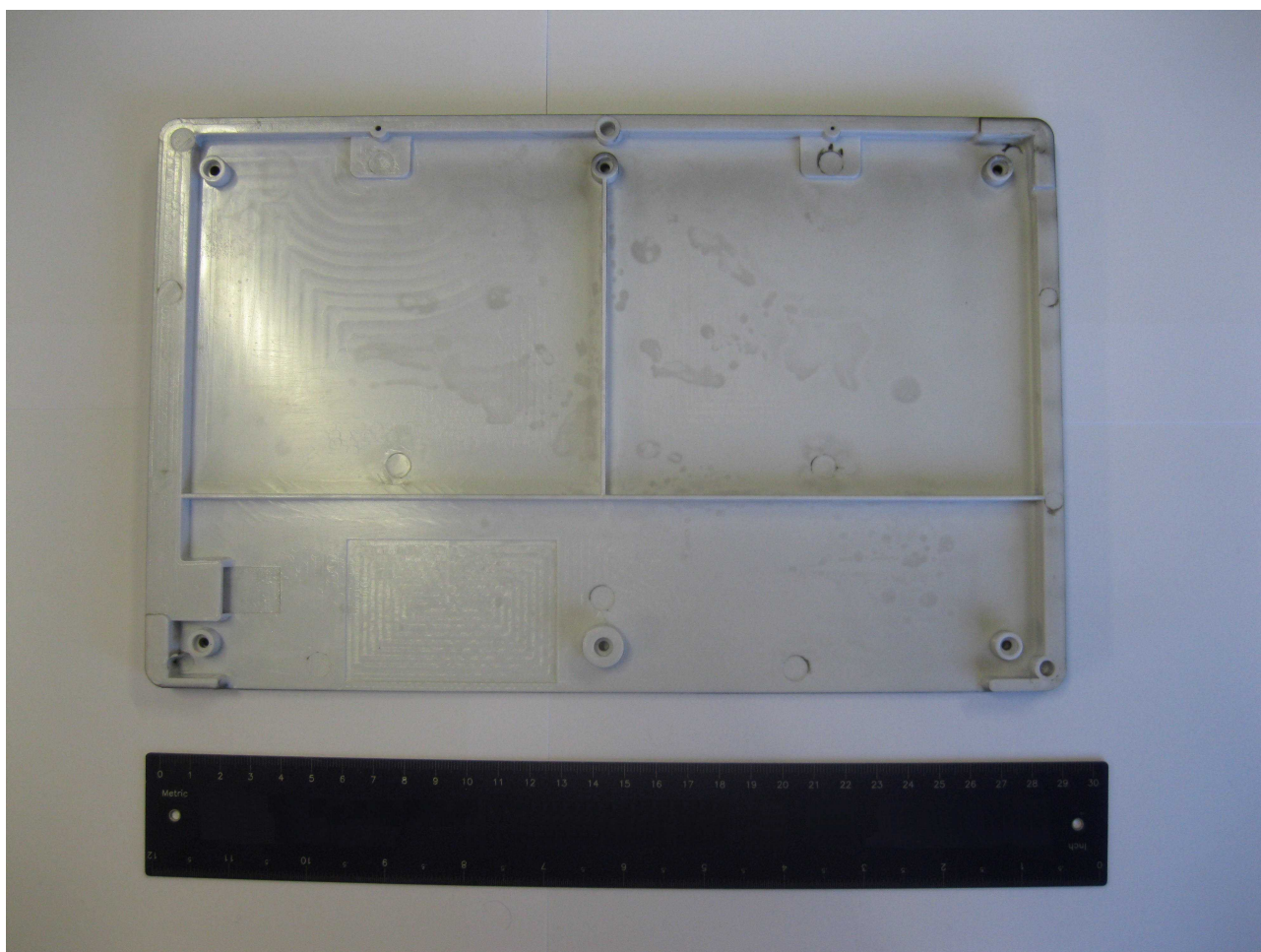
Figure 6: R1260UB –Bottom enclosure internal view
