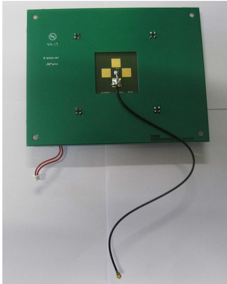
Figure 5: Antenna support and LED board – Bottom side
