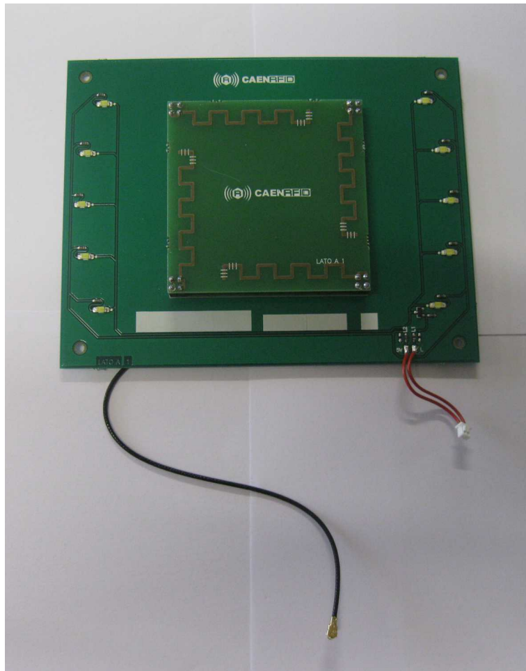
Figure 4: Antenna support and LED board - Top side
