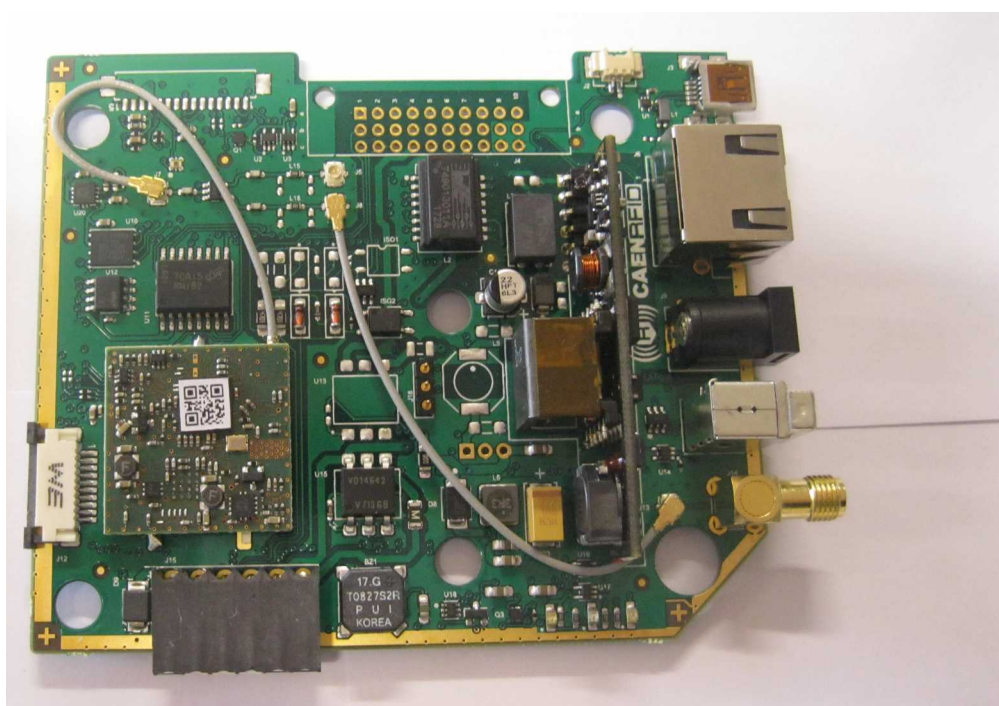
Figure 8: Main Board – Top side
