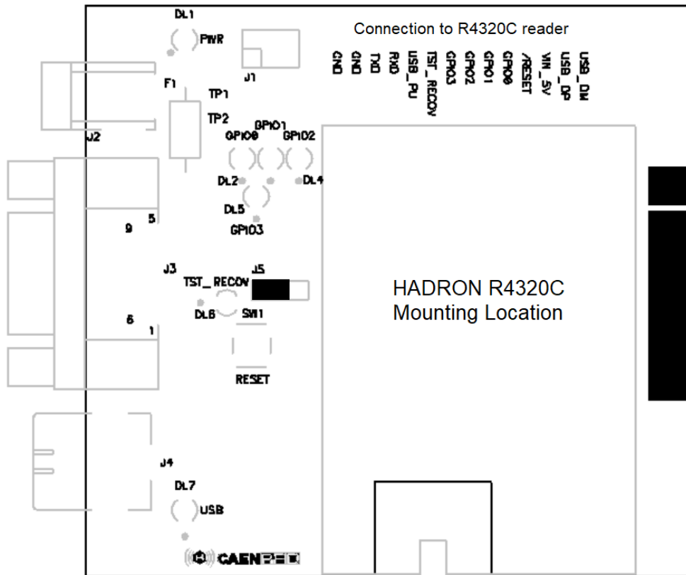
Fig. 3.3: Hadron R4320CEVB Technical Drawing
