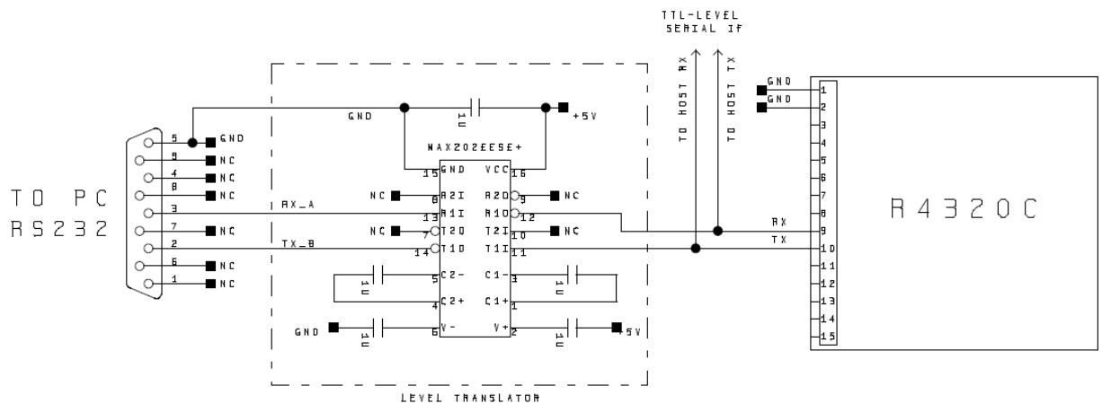
Fig. 2.5: Hadron R4320C RS232 Connection
