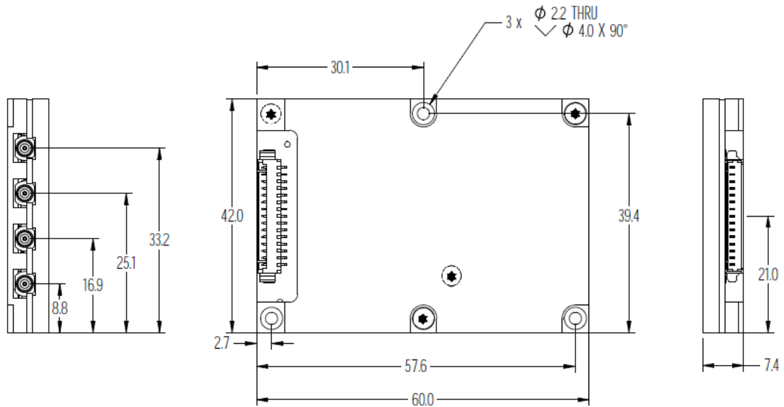
Physical dimensions: millimeters
