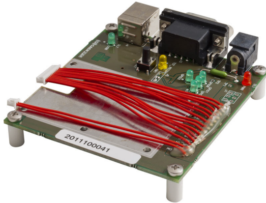
Fig. 1.3: Hadron R4320CEVB Evaluation Board
