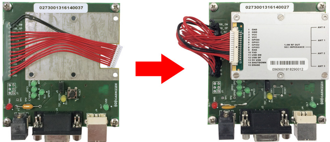
Fig. 3.2: Connection of the R4320C module to the R4320CEVB evaluation board
