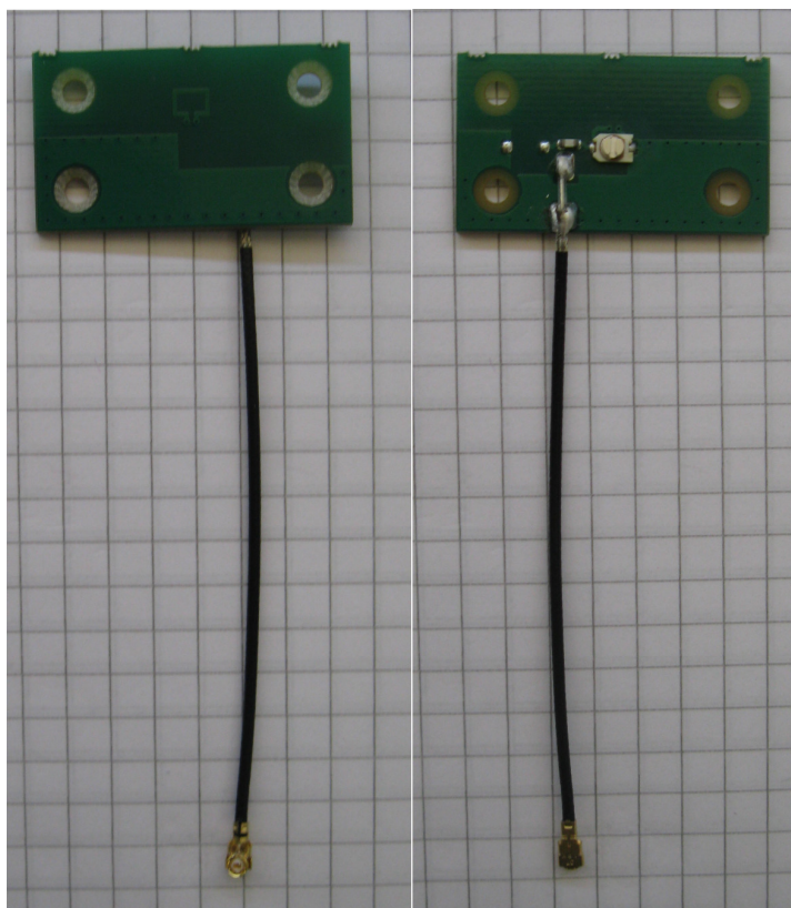
Figure 6: Antenna - Top and bottom view
