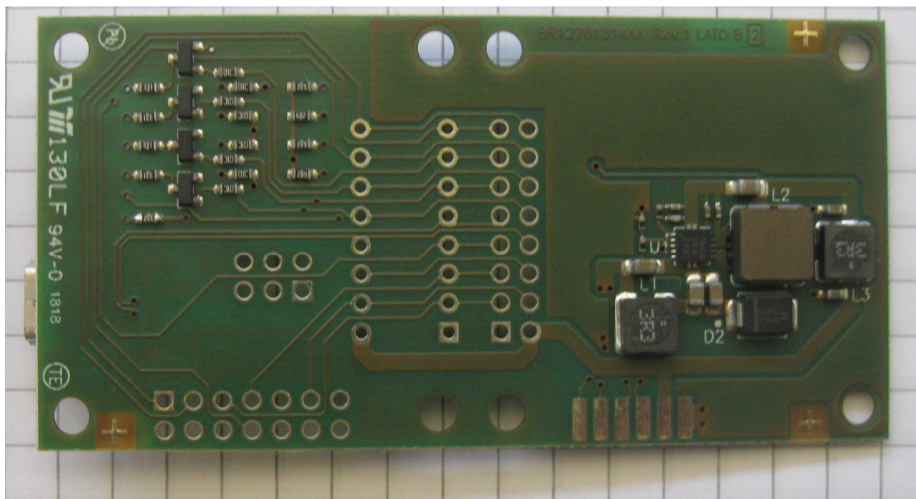
Figure 5: Interface board - Bottom View
