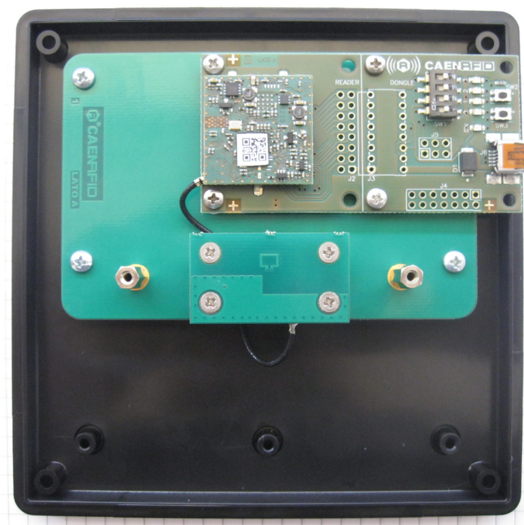
Figure 3: Internal View
