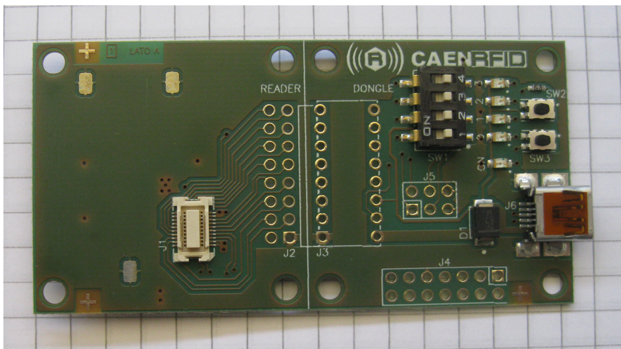
Figure 4: Interface board - Top View
