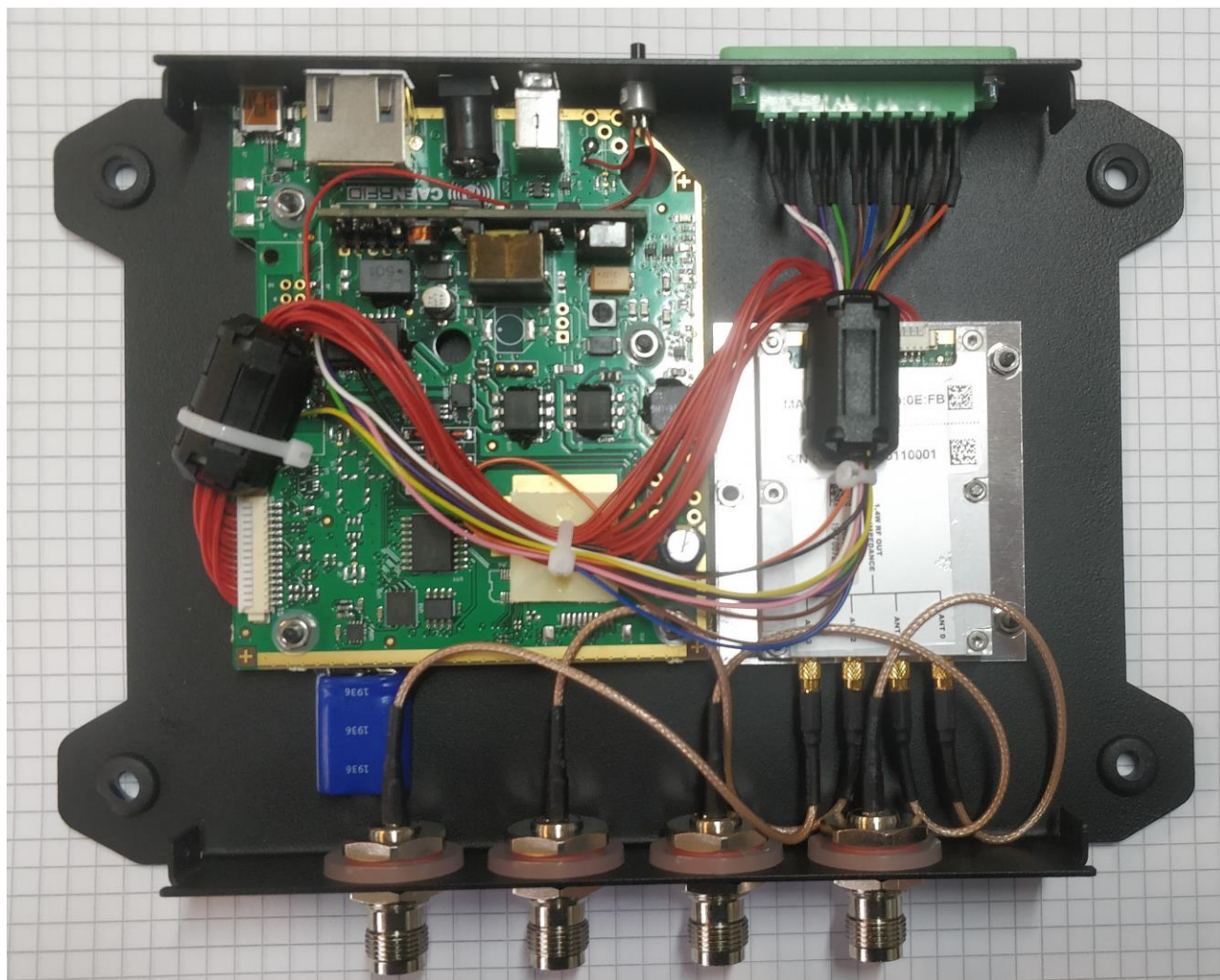
Fig. 3: Internal assembly
