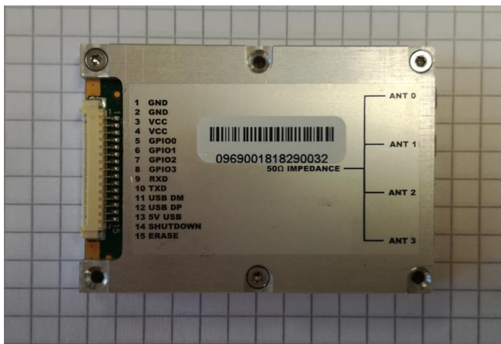
Fig. 7: RFID Module – External view - Bottom side
