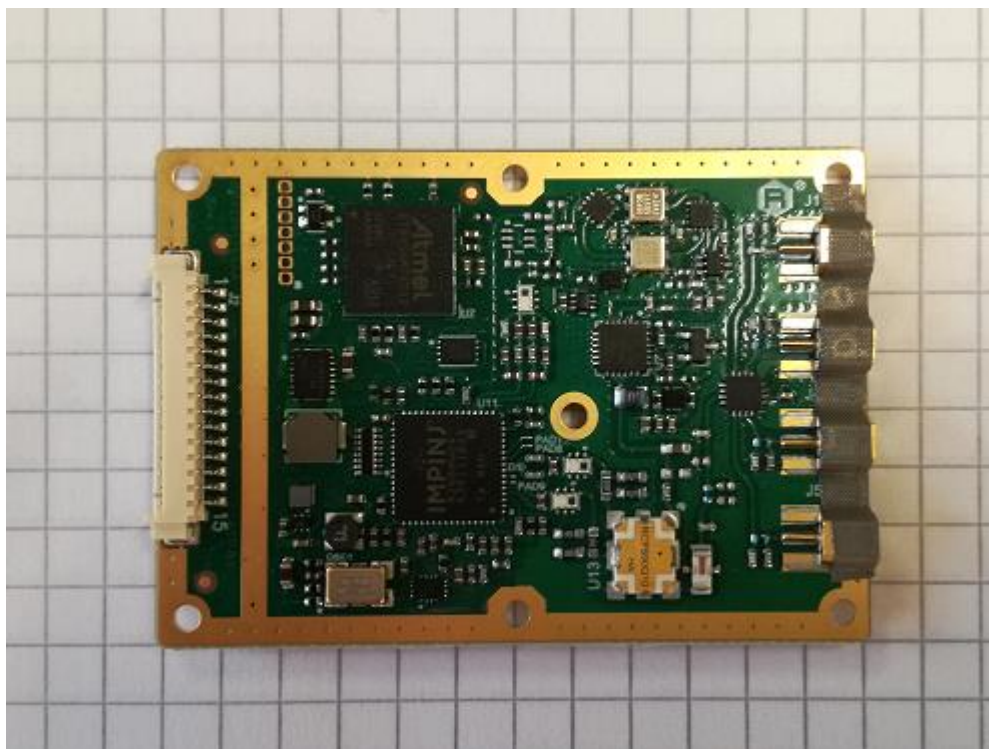
Fig. 4: RFID Module – Internal view - Top side
