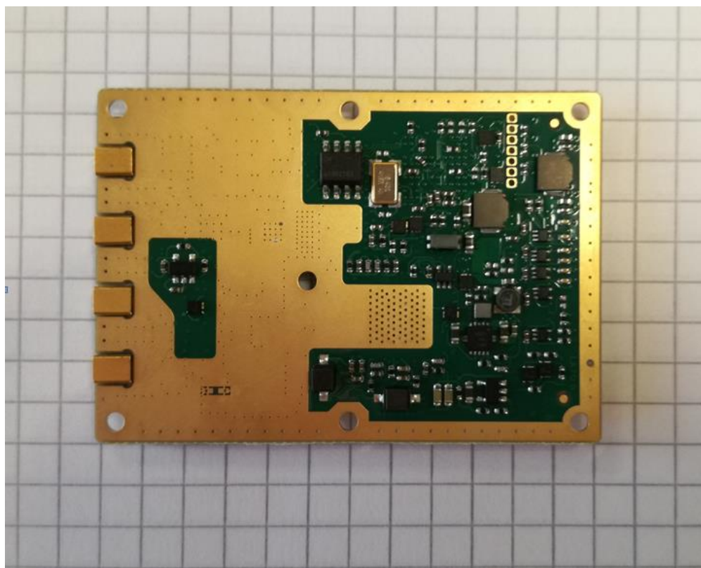
Fig. 5: RFID Module – Internal view - Bottom side
