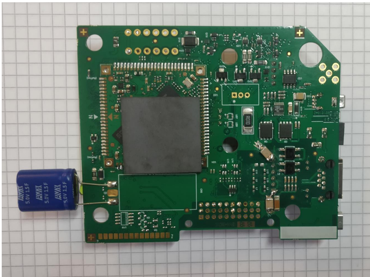
Fig. 2: Main Board - Bottom side
