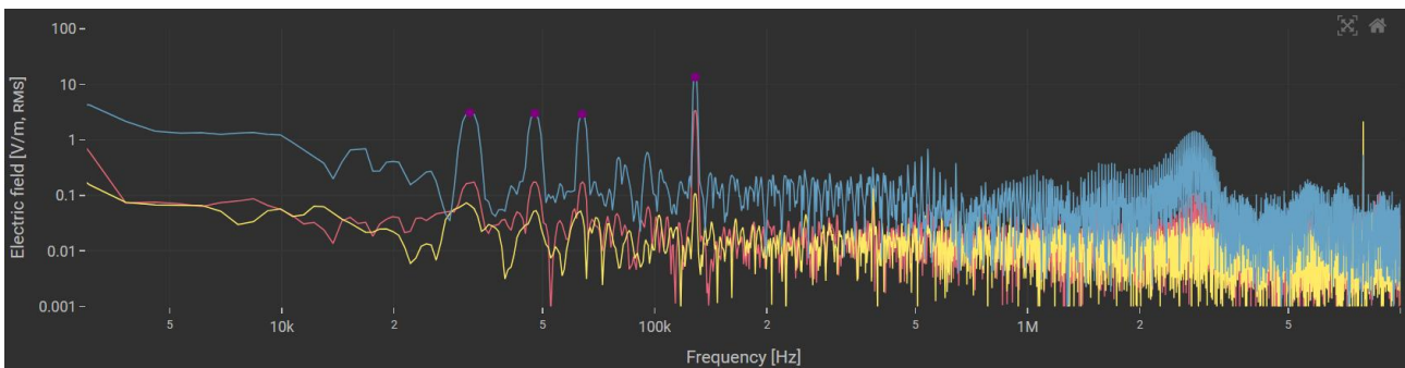
Figure 13. E-field frequency-domain plot from 3 kHz to 10 MHz
