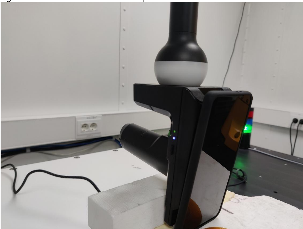
Figure 11. Front side of the DUT with a separation distance of 0mm
