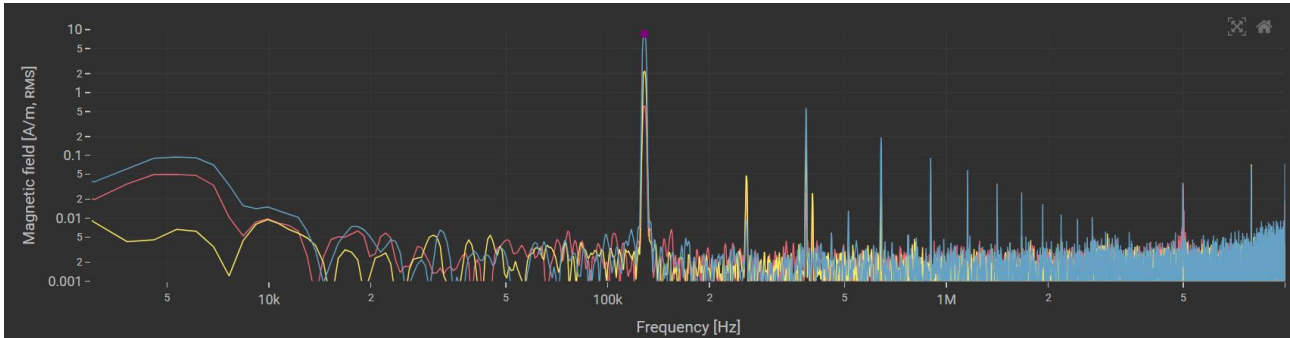
Figure 12. H-field frequency-domain plot from 3 kHz to 10 MHz
