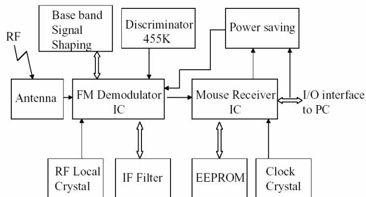
RF Mouse Receiver Function block
