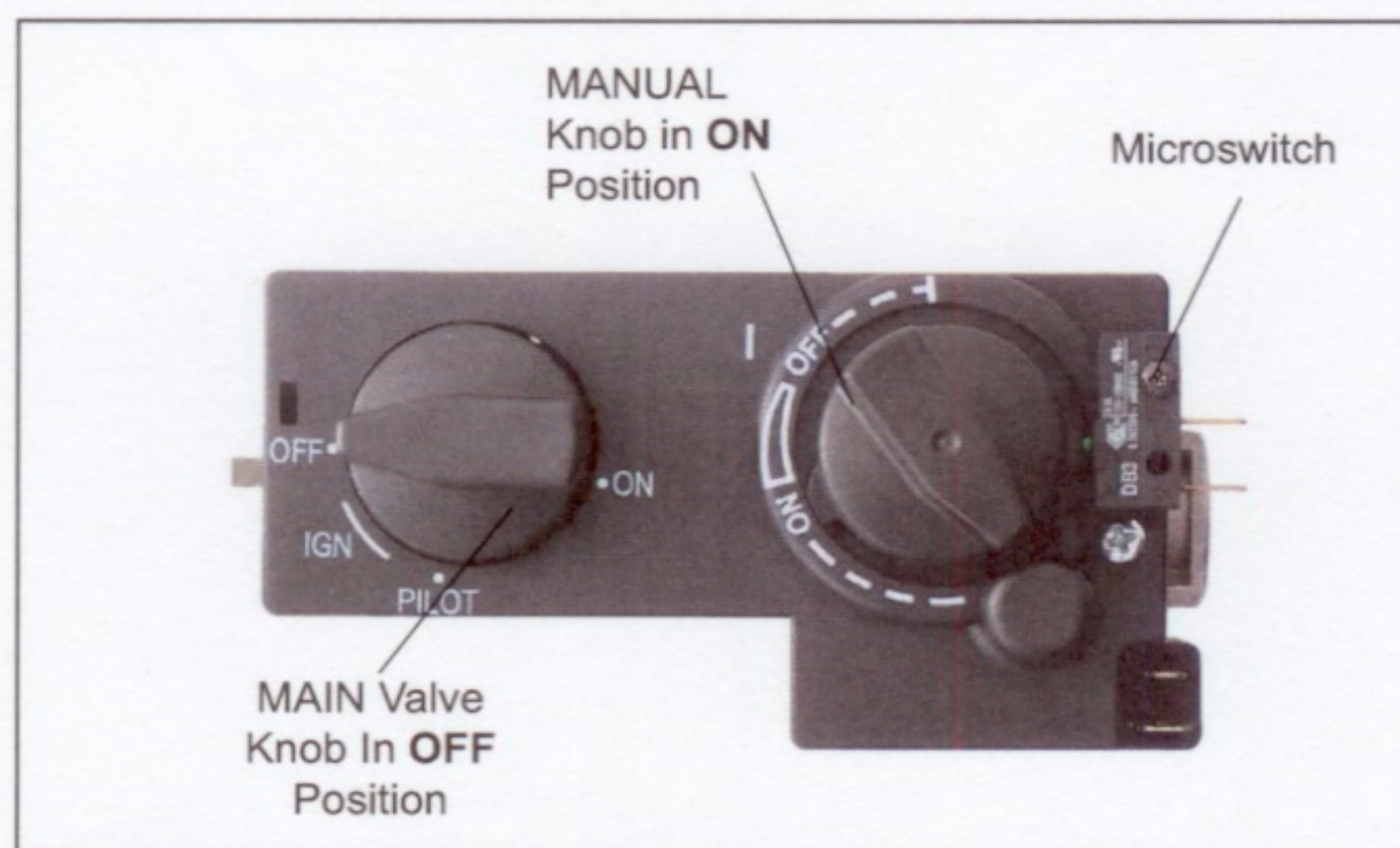
Figure 5: Combination Control
