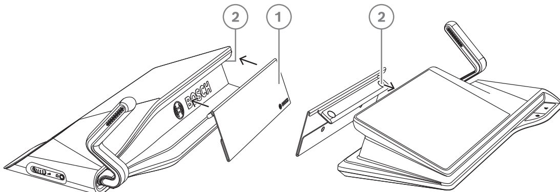
Figure 7.18: DCMN-NCH assembly
