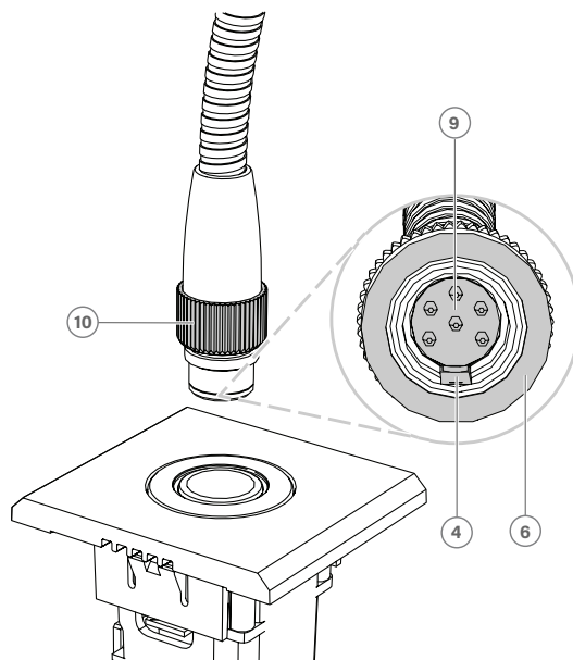
Figure 7.17: DCNM-MICSLL / DCNM-MICSLS connection
