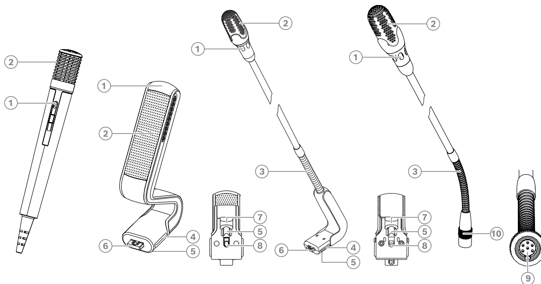
Figure 7.15: DCNM-FHH / DCNM-FHHC, DCNM-HDMIC, DCNM-MICS / DCNM-MICL and DCNM-MICSL/LS / DCNM-MICSL
