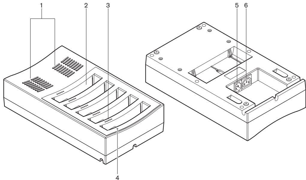
Figure 6.6: Charger DCNM-WCH05
