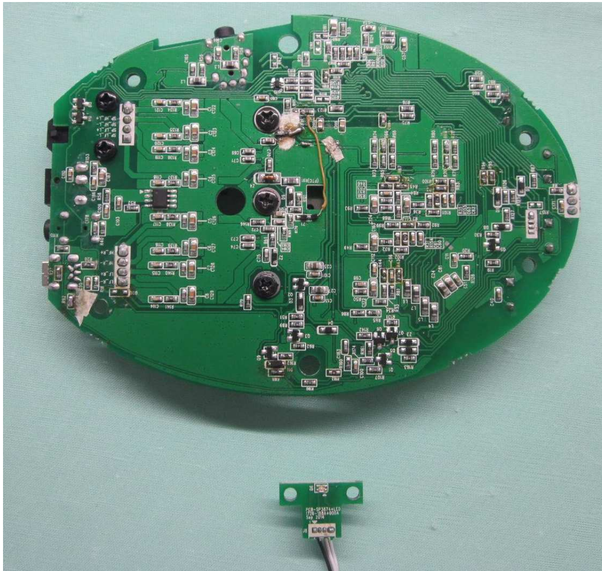
PHOTOGRAPH OF THE PRODUCT INNER CIRCUIT BOTTOM VIEW
