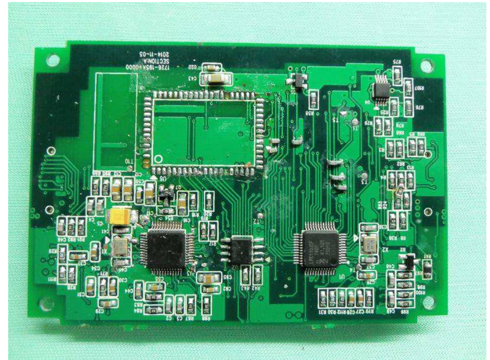
INNER CIRCUIT BOTTOM VIEW
