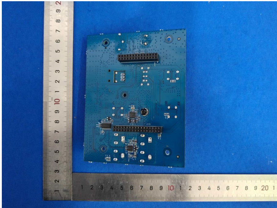
Figure 24: Main Board For Primary Speaker
