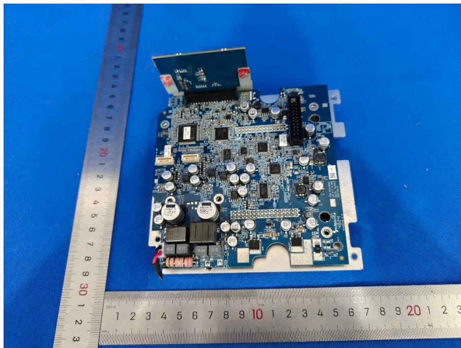
Figure 15: Main Board For Primary Speaker
