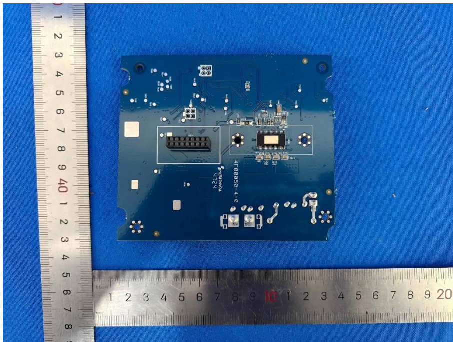
Figure 27: Main Board For Secondary Speaker
