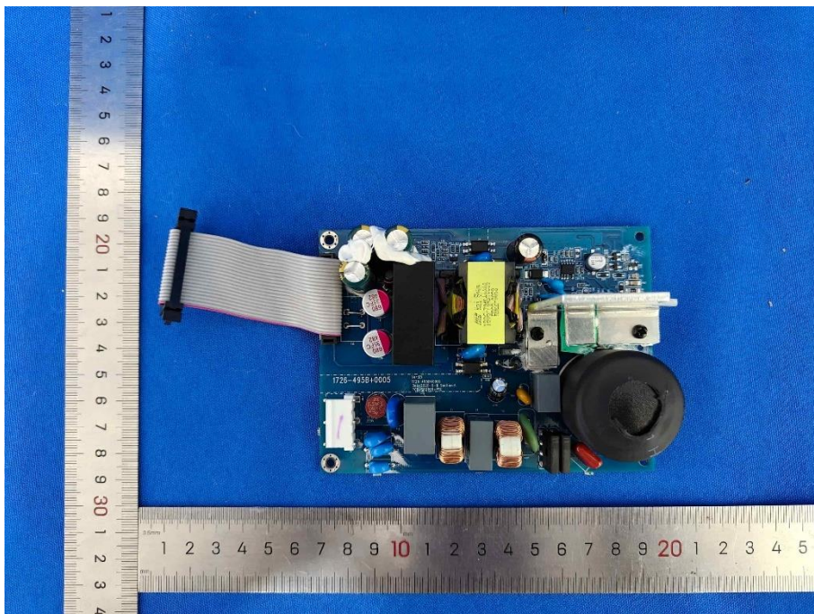
Figure 13: Power Board For Primary Speaker
