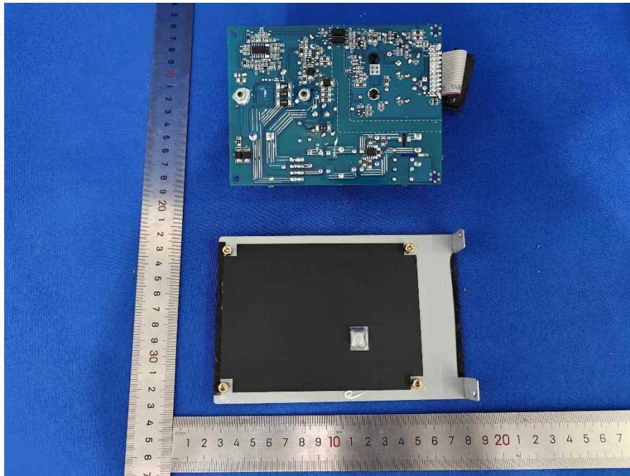
Figure 12: Power Board For Primary Speaker
