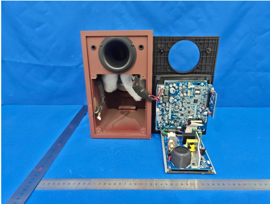
Figure 8: Primary Speaker Internal View
