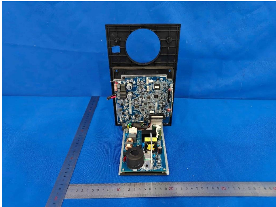
Figure 10: Primary Speaker Internal View
