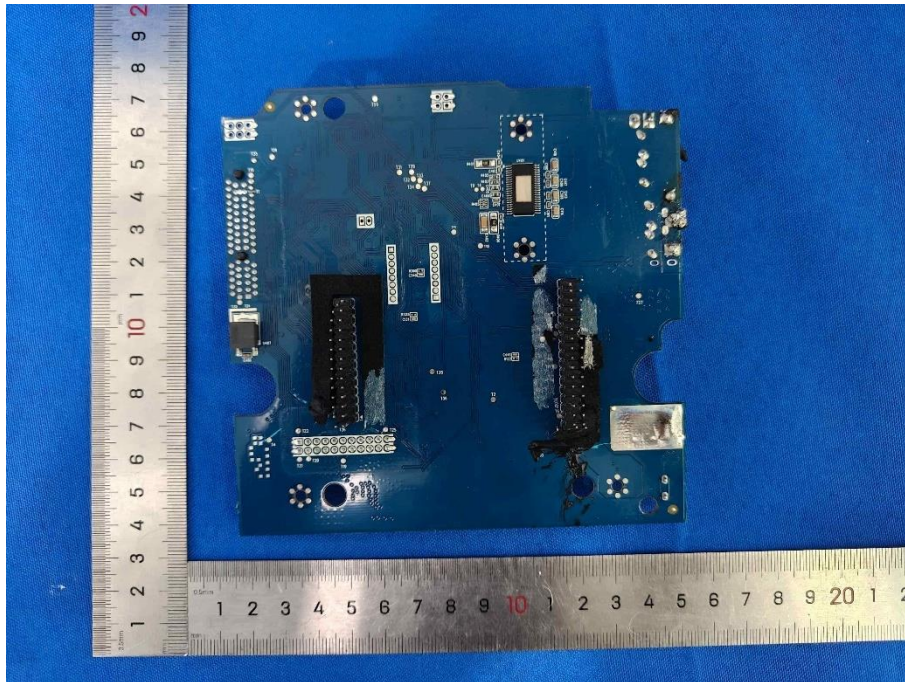
Figure 18: Main Board For Primary Speaker
