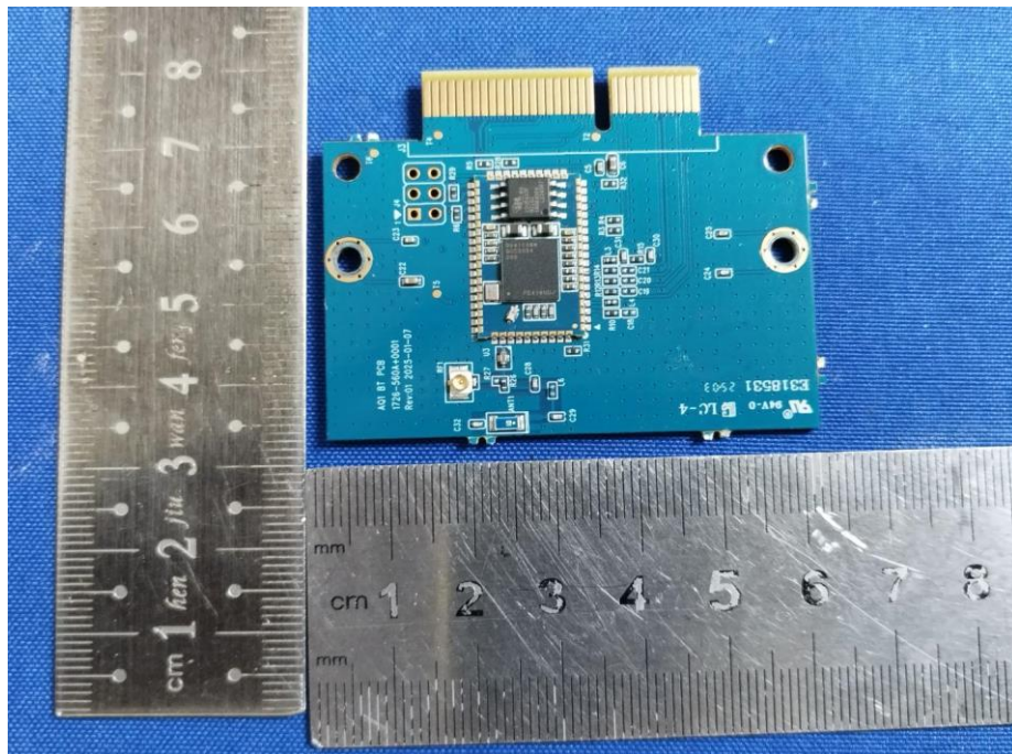
Figure 22: Main Board For Primary Speaker
