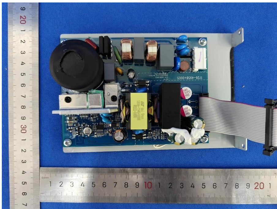
Figure 11: Power Board For Primary Speaker
