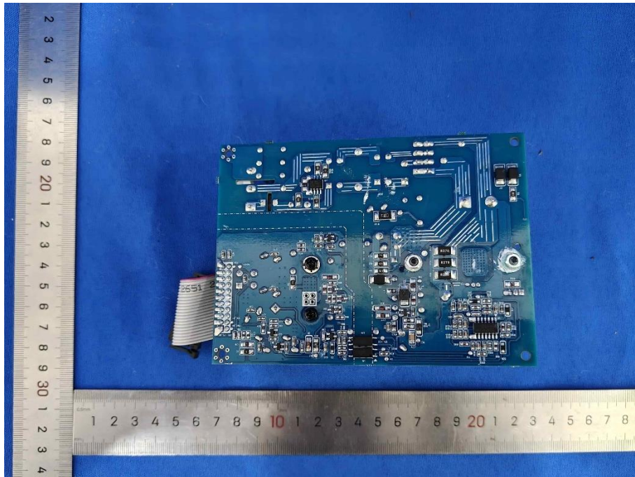
Figure 14: Power Board For Primary Speaker
