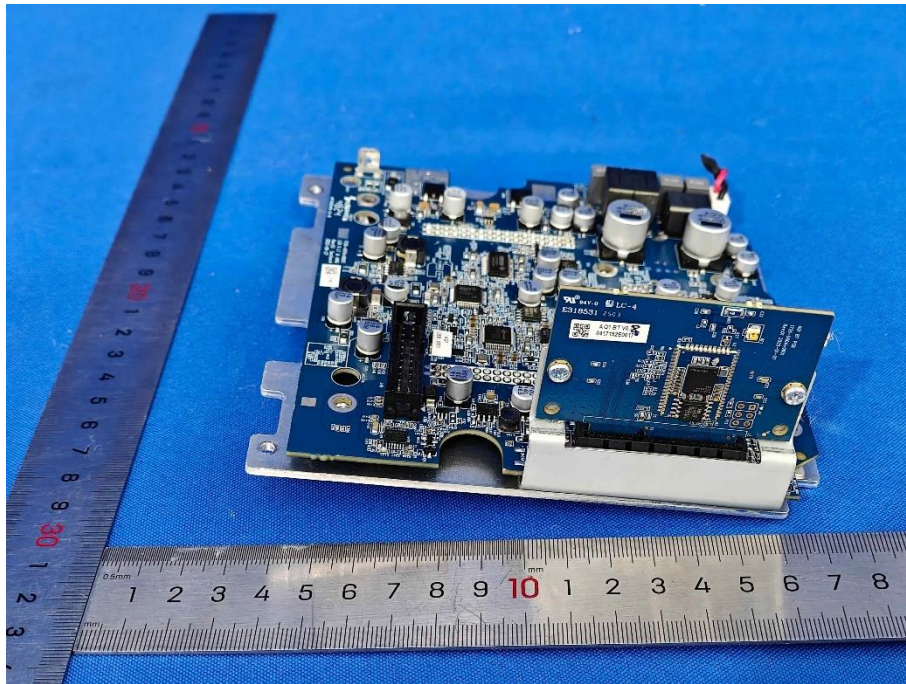
Figure 16: Main Board For Primary Speaker
