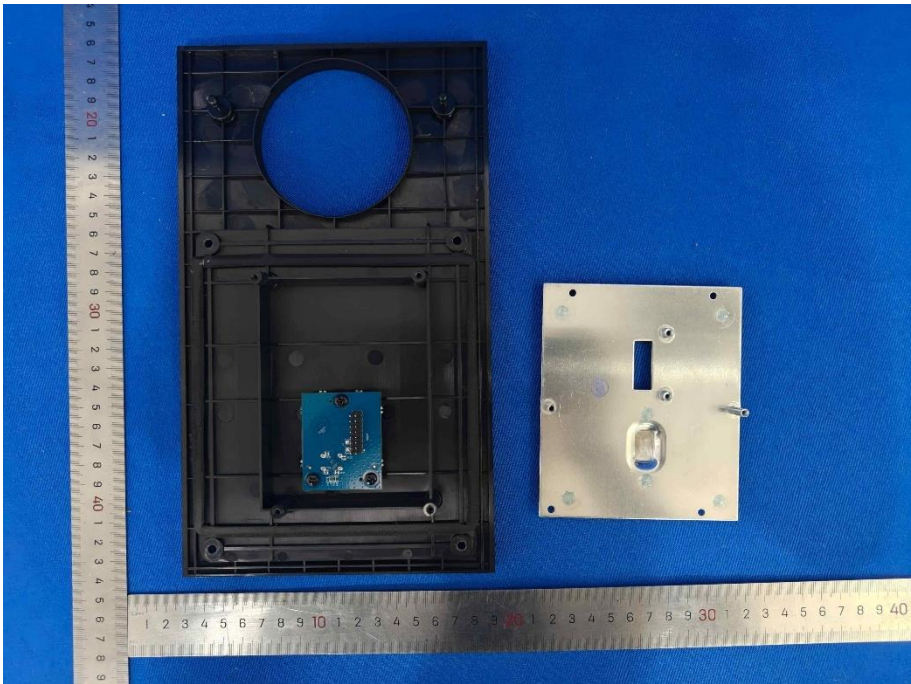
Figure 28: Secondary Speaker Internal View
