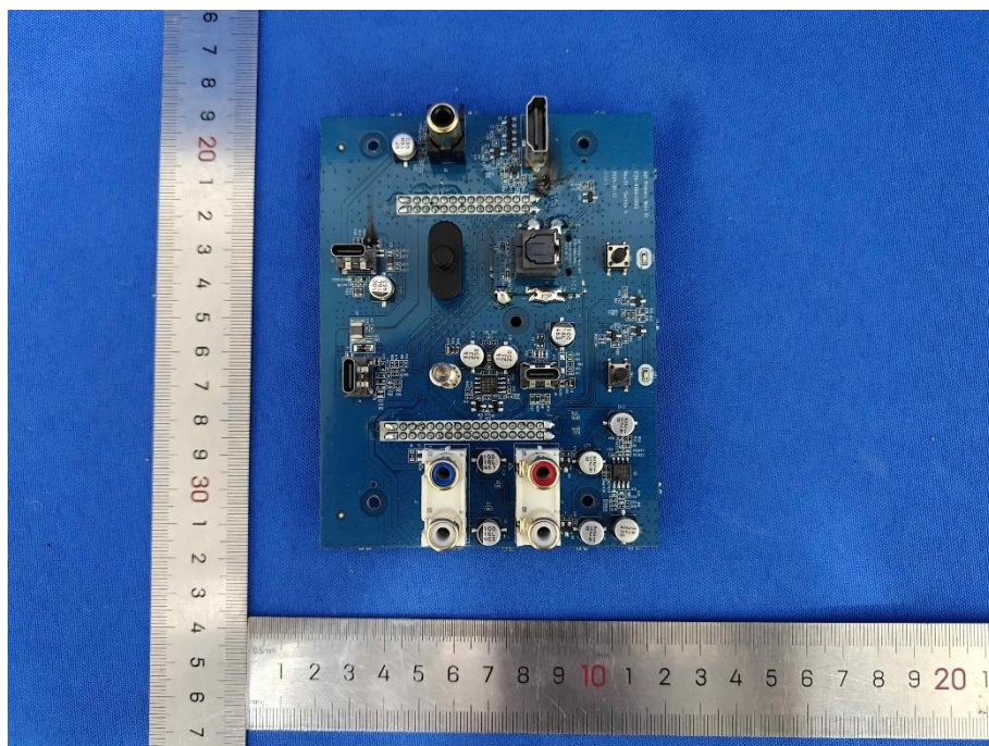
Figure 23: Main Board For Primary Speaker
