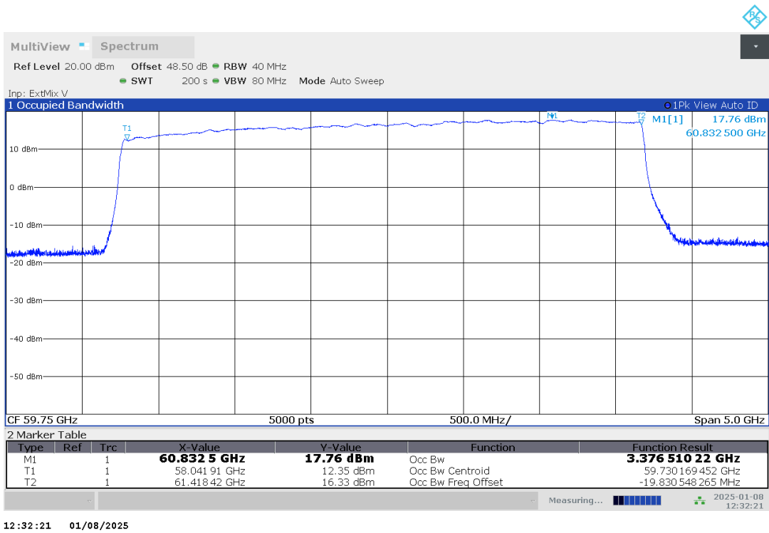
Plot no. 8: 99% OBW, Peak detector, -20 °C
