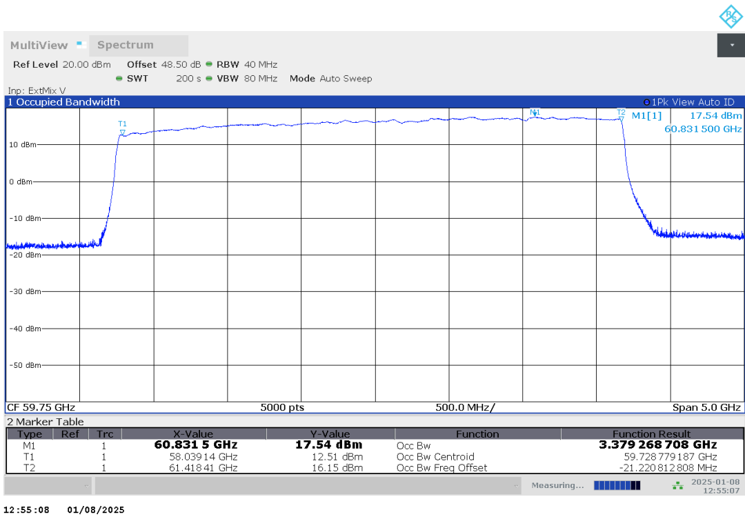
Plot no. 9: 99% OBW, Peak detector, -10 °C
