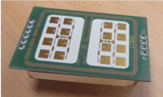
picture 1 EUT back
