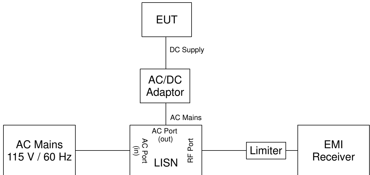
SCHEMATIC TEST SETUP
