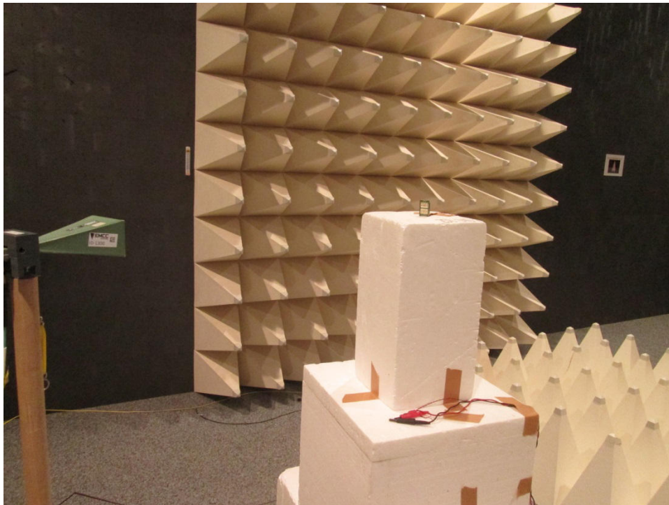
Photograph A1-9: Sample setup photo of radiated emissions 18 – 26.5 GHz at 1 m distance
