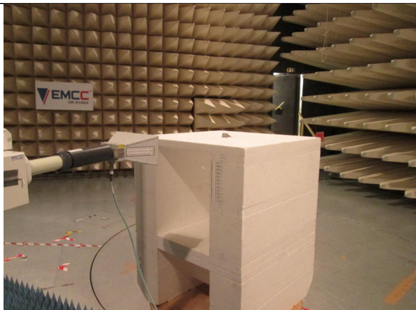
Sample photo of setup showing a different EUT (IPS-354)
