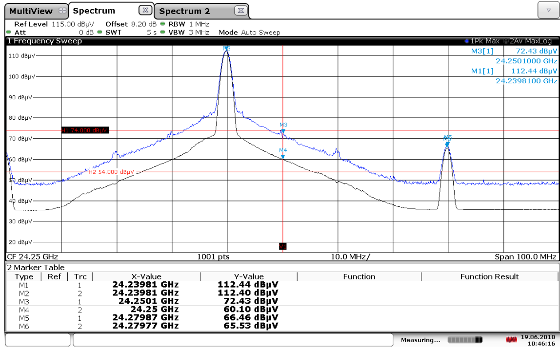
Plot No. 25: Band-Edge-Compliance, upper band-edge, stopped mode, high frequency, S/N: 00000103
