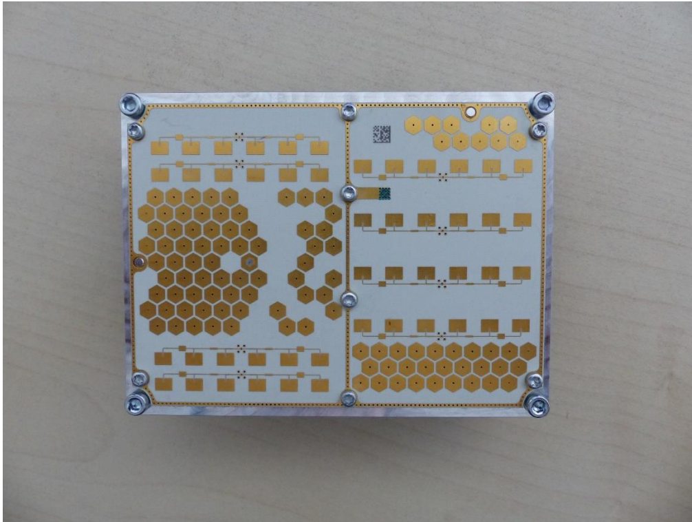
Photo 3: DUT front side
