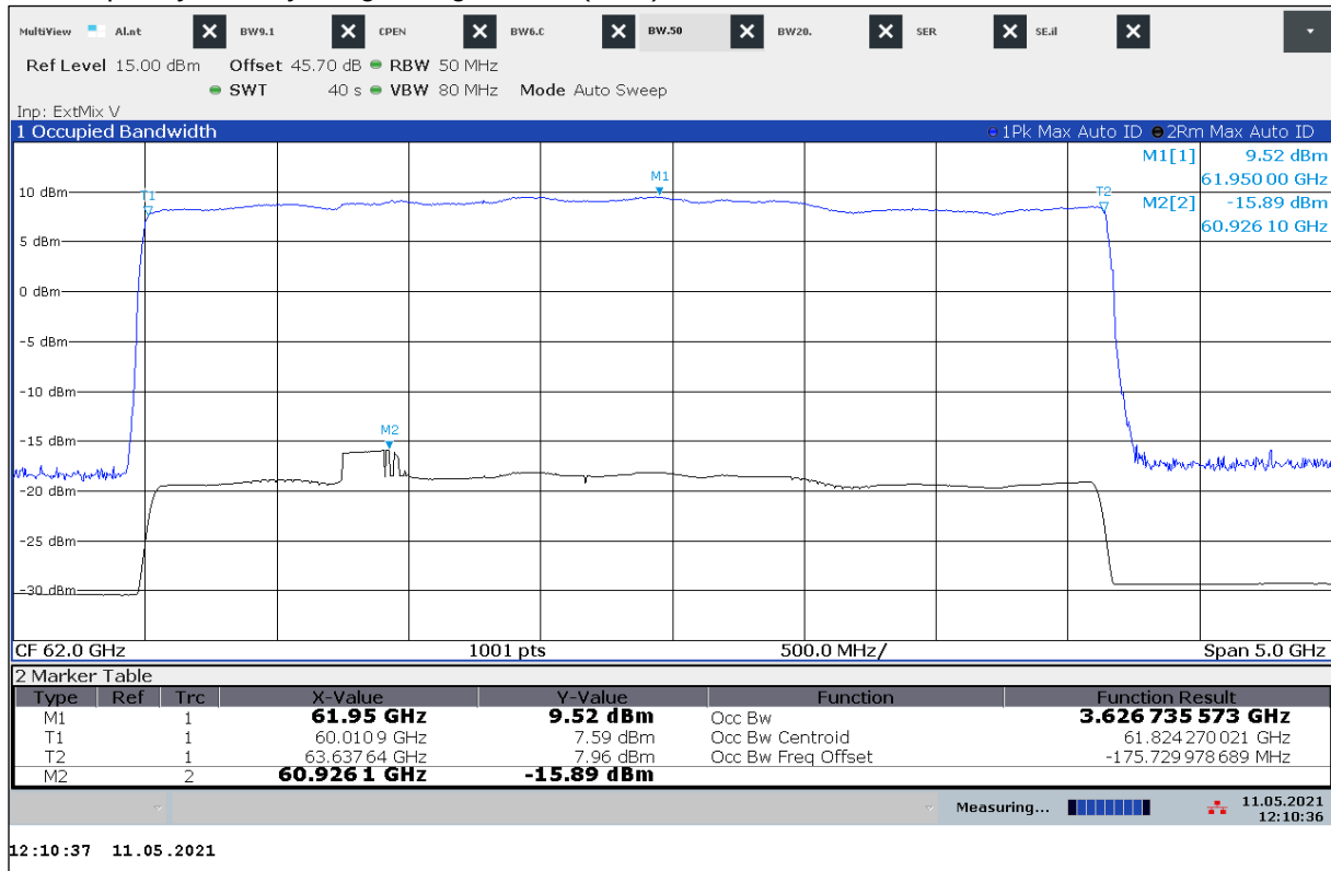
Plot 37: Frequency Stability, Single Target Mode (STM), -30 °C / V min-max
