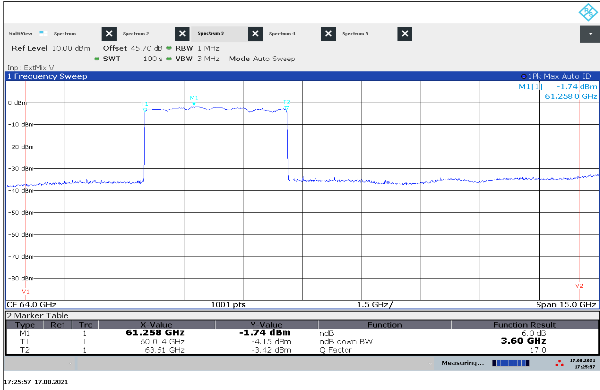
Plot 3: Multi Target Mode 10 Hz (MTM10), 99%, N6dB OBW
