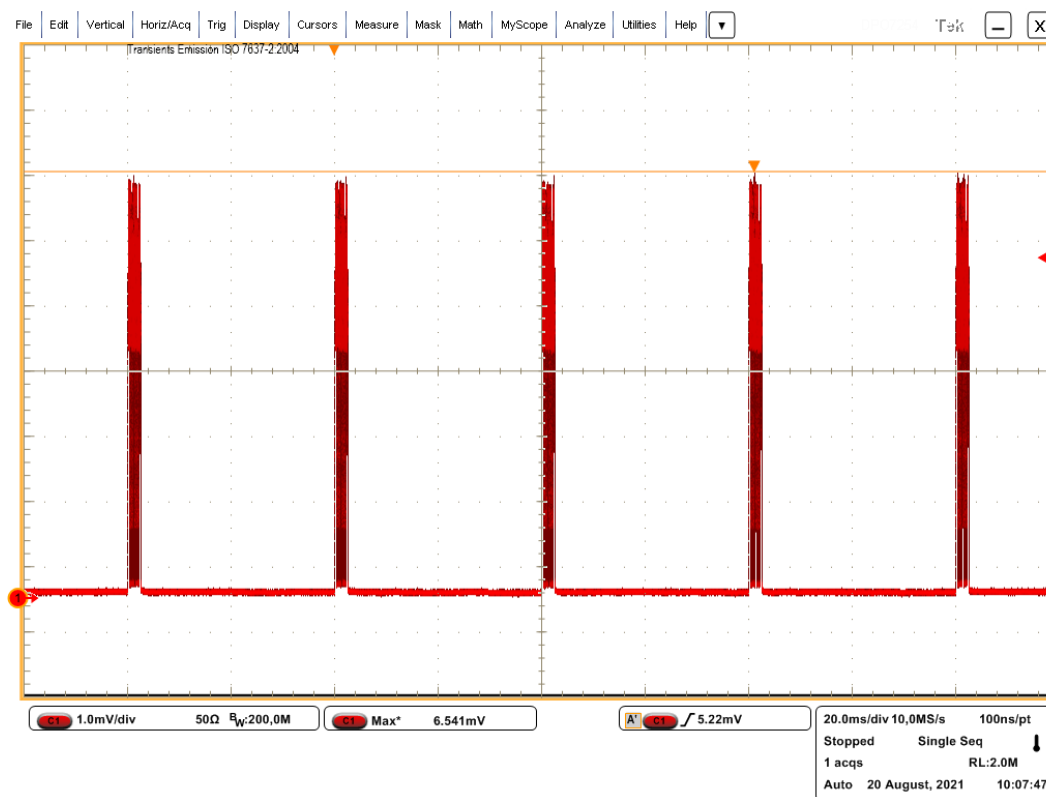
Plot 12: Multi Target Mode 25 Hz (MTM25), RF-detector measurement
