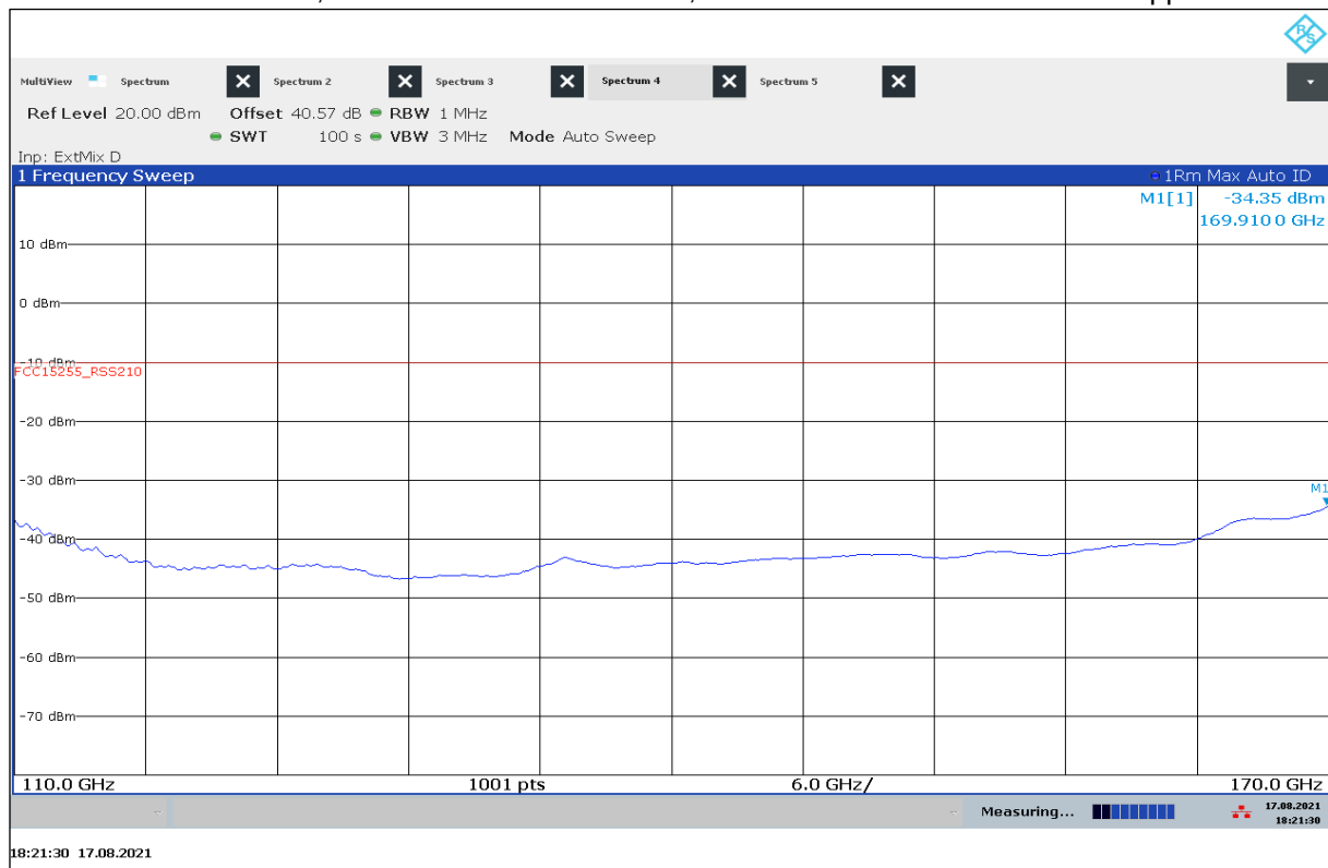
Plot 32: 110 GHz – 170 GHz, antenna vertical / horizontal, valid for all modulations and all stopped mode
