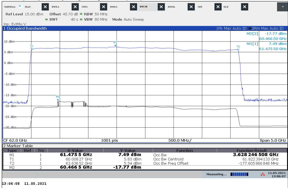
Plot 41: Frequency Stability, Single Target Mode (STM), 10 °C / V min-max
