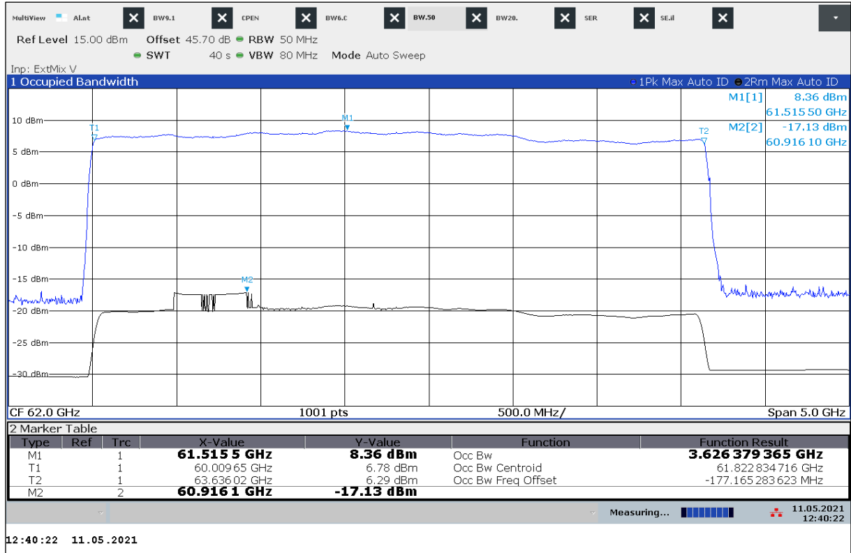
Plot 40: Frequency Stability, Single Target Mode (STM), 0 °C / V min-max
