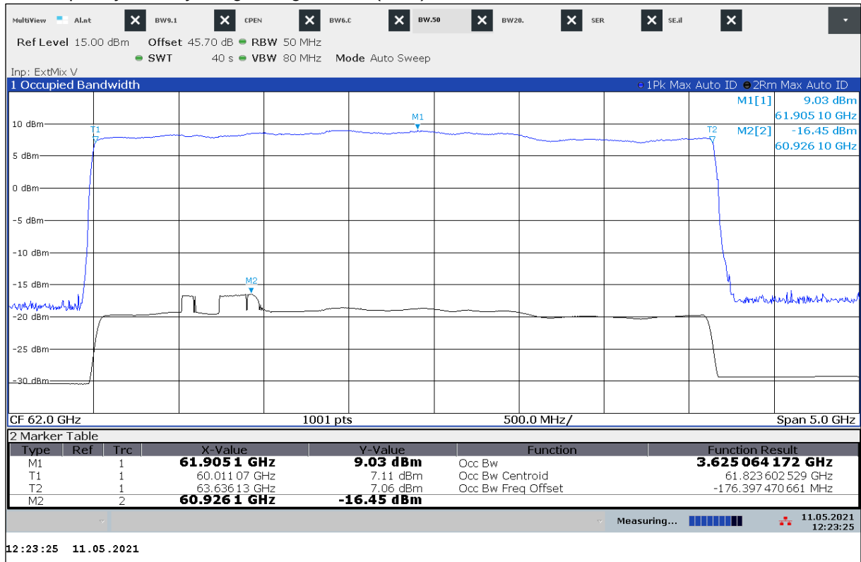
Plot 39: Frequency Stability, Single Target Mode (STM), -10 °C / V min-max
