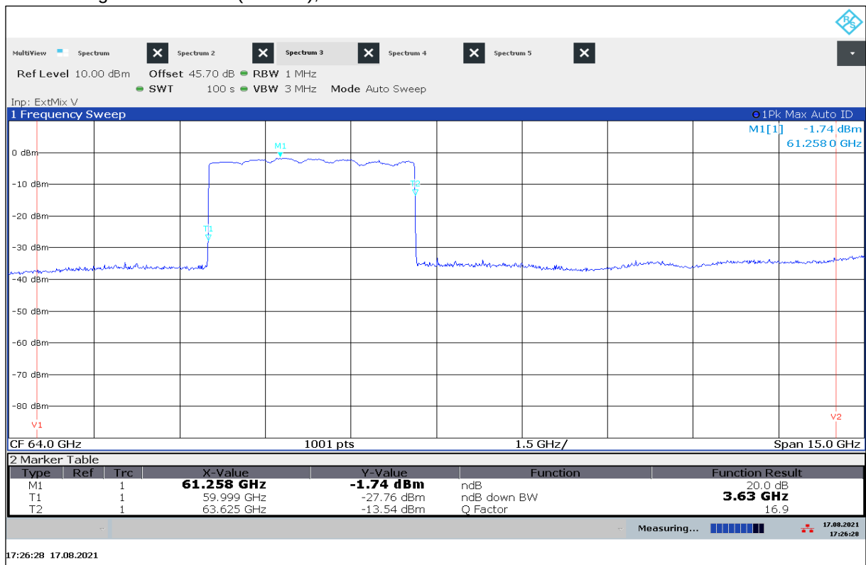
Plot 4: Multi Target Mode 10 Hz (MTM10), N20dB OBW
