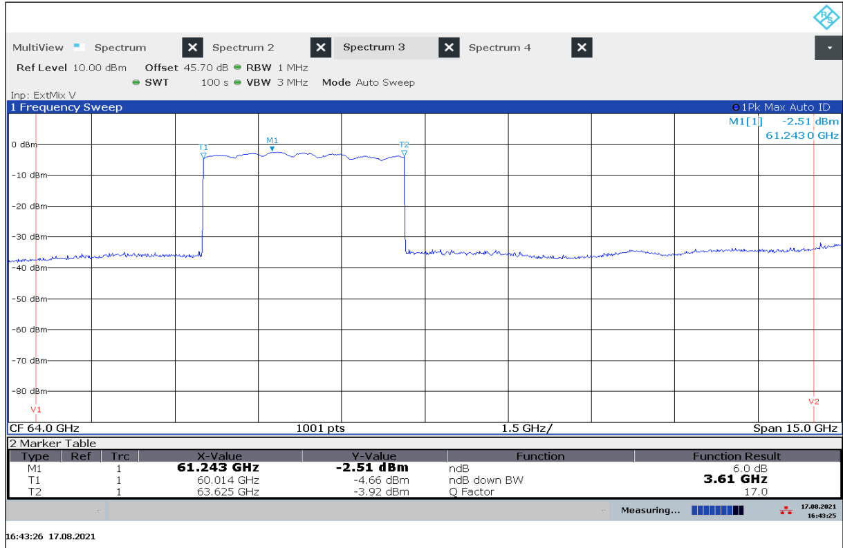
Plot 7: Multi Target Mode 25 Hz (MTM25), 99%, N6dB OBW
