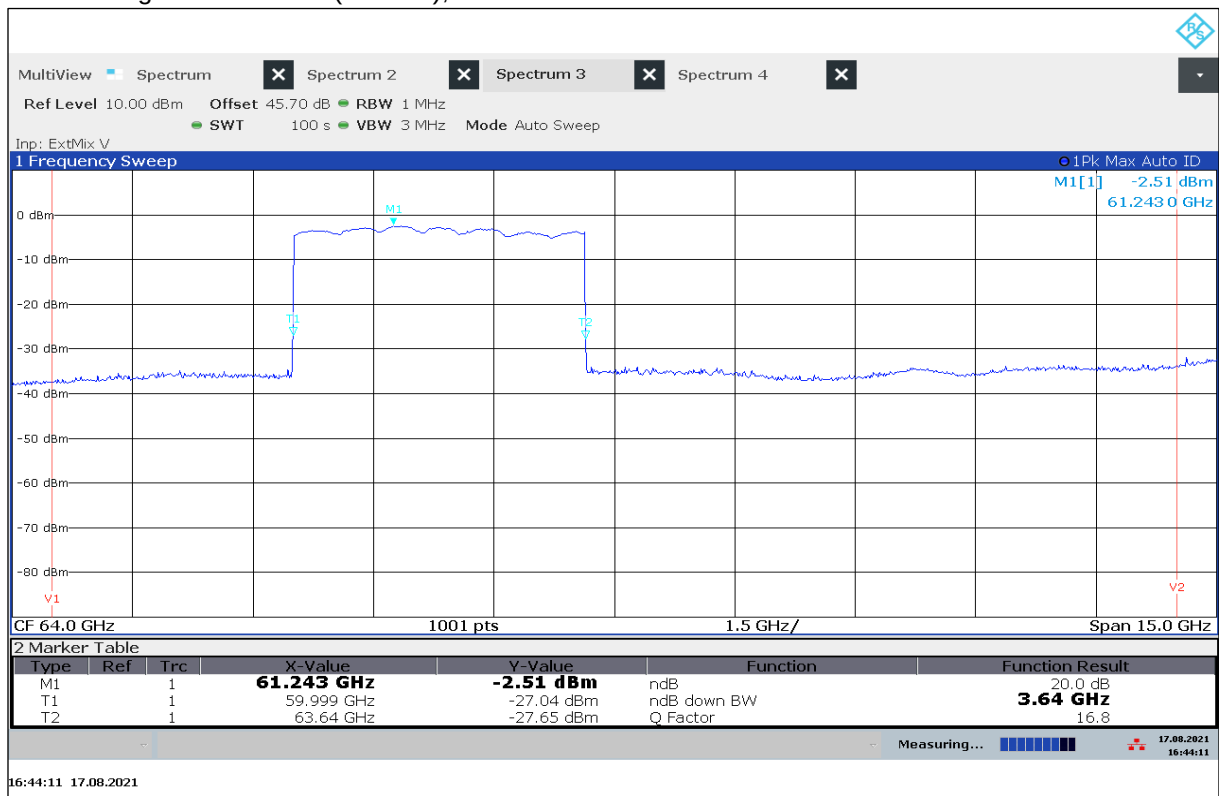
Plot 8: Multi Target Mode 25 Hz (MTM25), N20dB OBW
